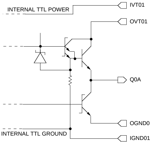
Figure 1. Output Structure
