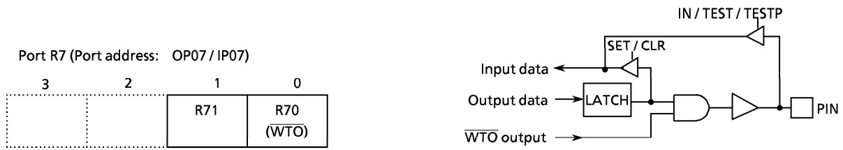
Figure 3-4. Ports R7
