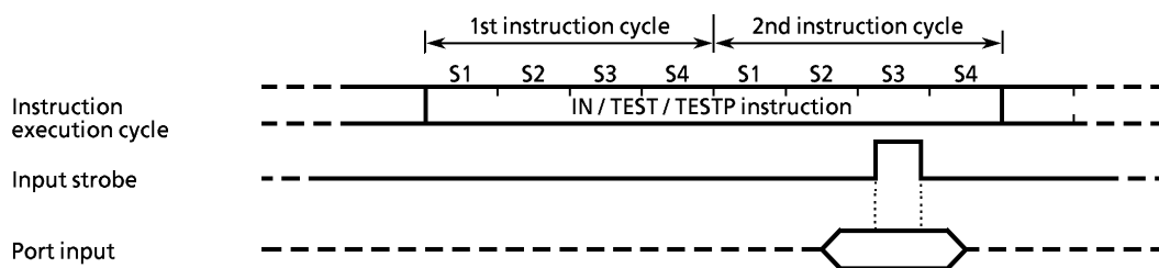
Figure 3-1. Input Timing
