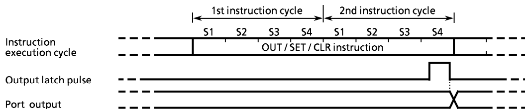
Figure 3-2. Output Timing
