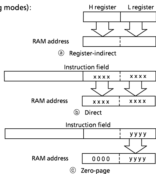
Figure 2-5. Addressing mode
