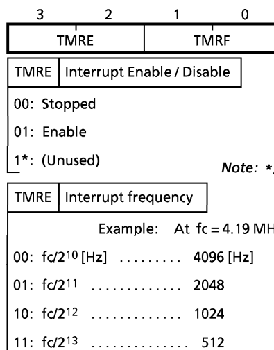
Figure 3-7. Command Register
