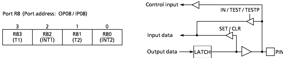
Figure 3-5. Port R8
