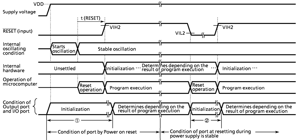
Figure 3-16. Port condition by Reset operation
