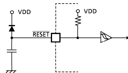
Figure 2-23. Simplified Power-On-Reset
