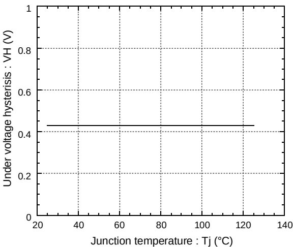
Under voltage hysteresis vs. Jnction temperature
