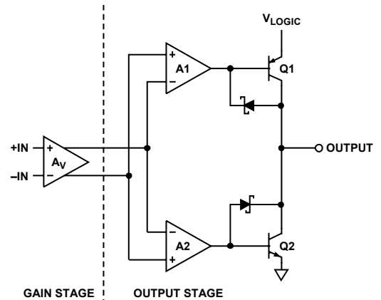
Figure 9. Simplified Schematic Diagram of TTL-/CMOS-Compatible Output Stage
