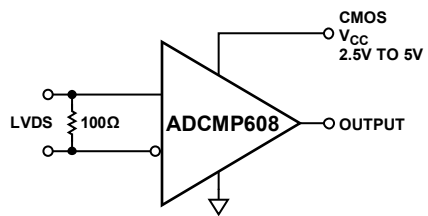
Figure 13. LVDS-to-CMOS Receiver
