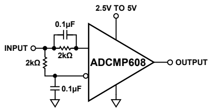
Figure 12. Self-Biased, 50% Slicer
