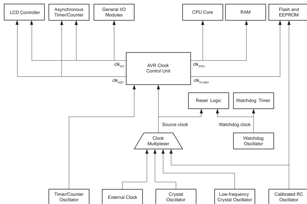
Figure 11. Clock Distribution
