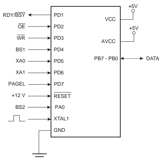
Figure 118. Parallel Programming
