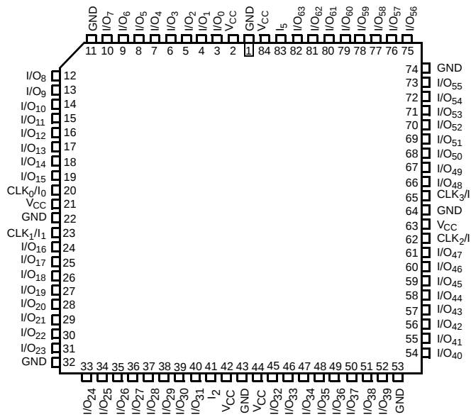
PLCC/CLCC Top View
