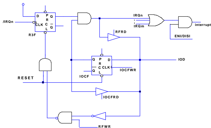
Fig. 9 Interrupt Input Circuit
