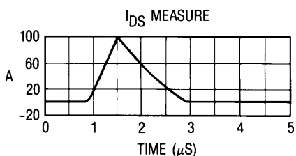
Figure 7. – Typical Transient Response of Rad Hard HEXFET During 1 \times 10^{12} Rad (Si)/Sec Exposure.
