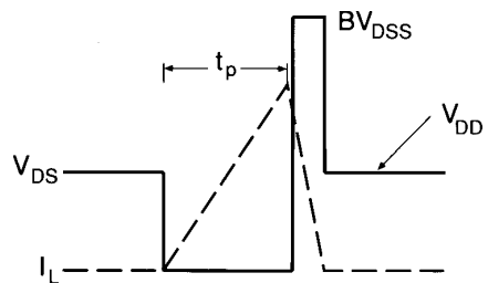
Figure 29b – Unclamped Inductive Waveforms
