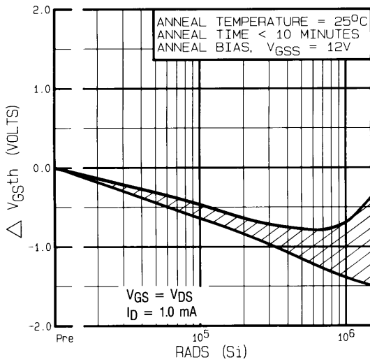
Figure 1. – Typical Response of Gate Threshold Voltage Vs. Total Dose Exposure.
