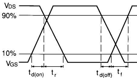
Figure 28b – Switching Time Waveforms
