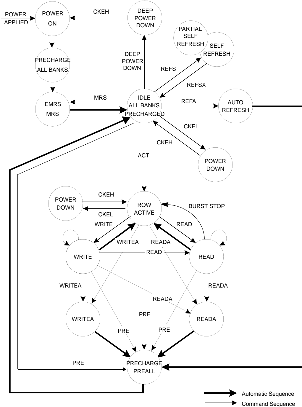
Figure.1 State diagram
