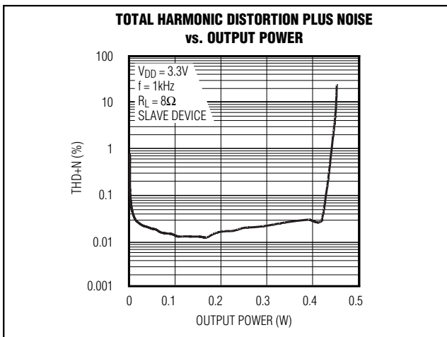
Figure 8. Master-Slave THD
