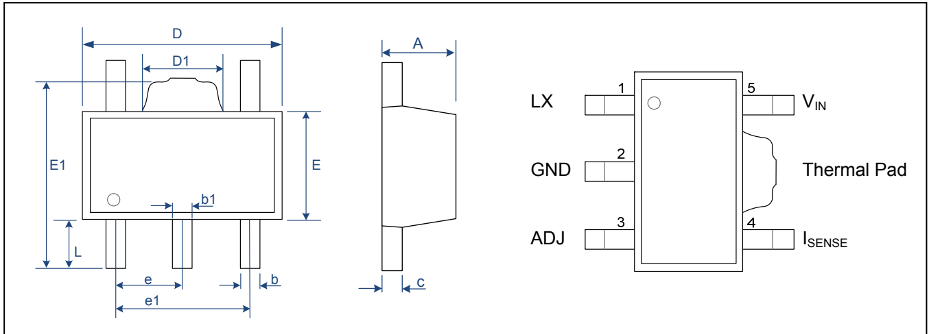
Figure 6.1 Pin Configuration and Package Drawing SOT89-5
