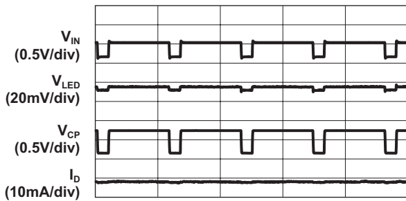
Line Response (1X Mode, 3x19mA Load)
