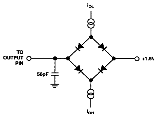
Figure 22. Equivalent Device Loading for AC Measurements (Except Output Enable/Disable)
