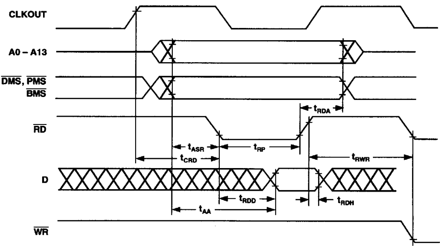
Figure 42. Memory Read
