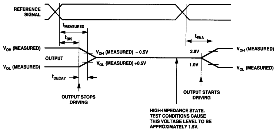
Figure 21. Output Enable/Disable
