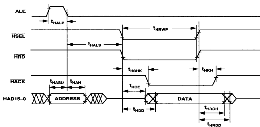
Figure 37. Host Interface Port (HMD1 = 1, HMD0 = 0)
