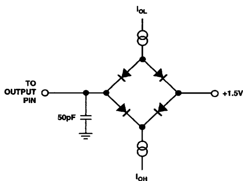
Figure 16. Equivalent Device Loading for AC Measurements (Except Output Enable/Disable)
