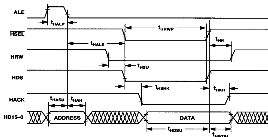
Host Write Cycle
