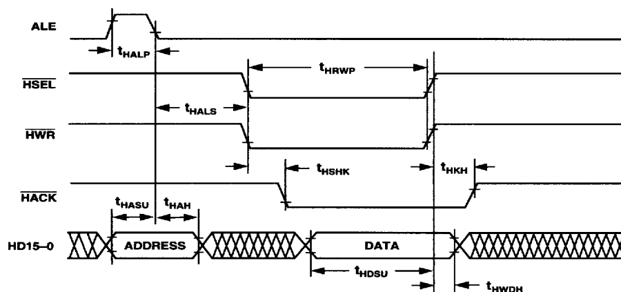
Host Write Cycle
