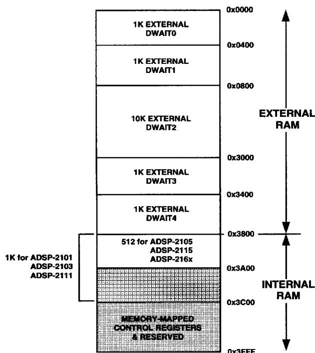
Figure 10. Data Memory Map (All Processors)
