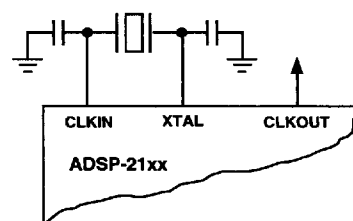
Figure 2. External Crystal Connections
