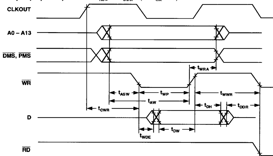
Figure 33. Memory Write
