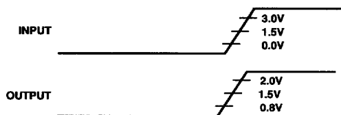
Figure 14. Voltage Reference Levels for AC Measurements (Except Output Enable/Disable)
