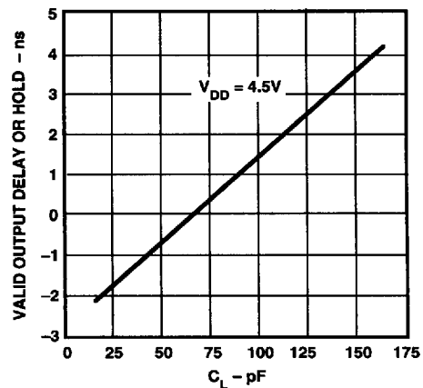
Figure 13. Typical Output Valid Delay or Hold vs. Load Capacitance, C_L (at Maximum Ambient Operating Temperature)
