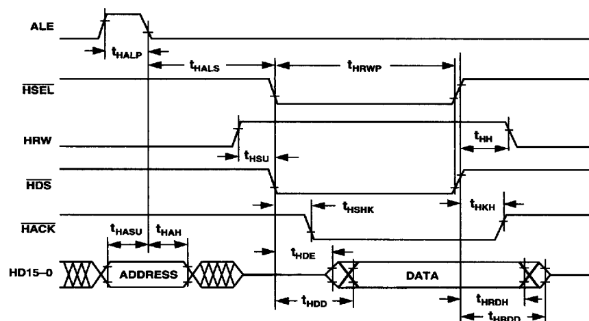
Figure 38. Host Interface Port (HMD1 = 1, HMD0 = 1)
