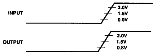
Figure 20. Voltage Reference Levels for AC Measurements (Except Output Enable/Disable)
