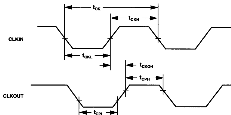
Figure 39. Clock Signals
