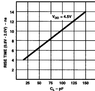
Figure 18. Typical Output Rise Time vs. Load Capacitance, C_L (at Maximum Ambient Operating Temperature)
