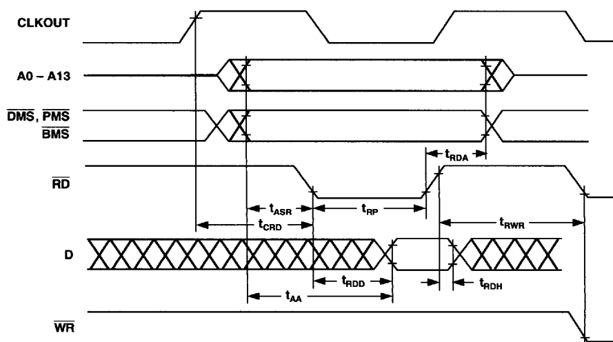
Figure 32. Memory Read
