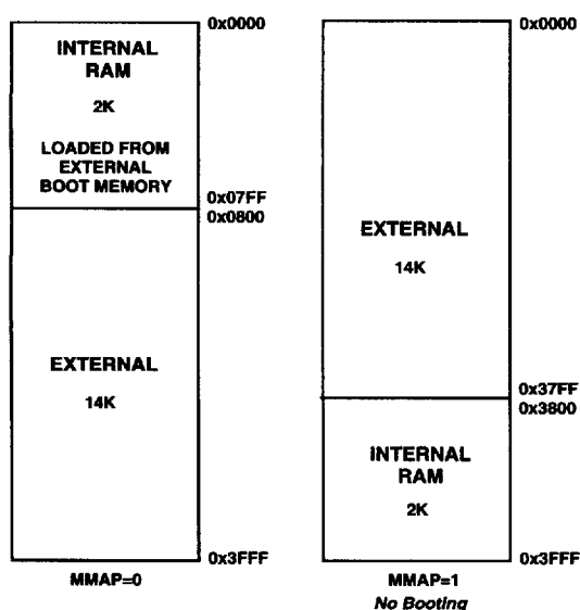
Figure 6. ADSP-2101/ADSP-2103/ADSP-2111 Program Memory Maps
