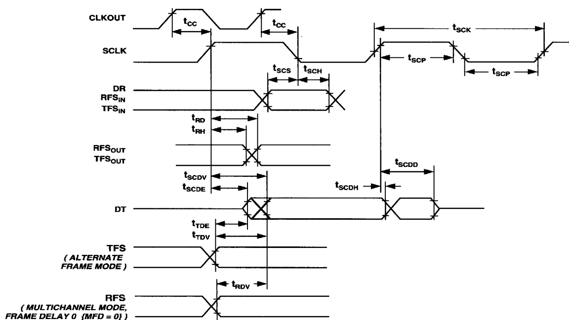
Figure 34. Serial Ports
