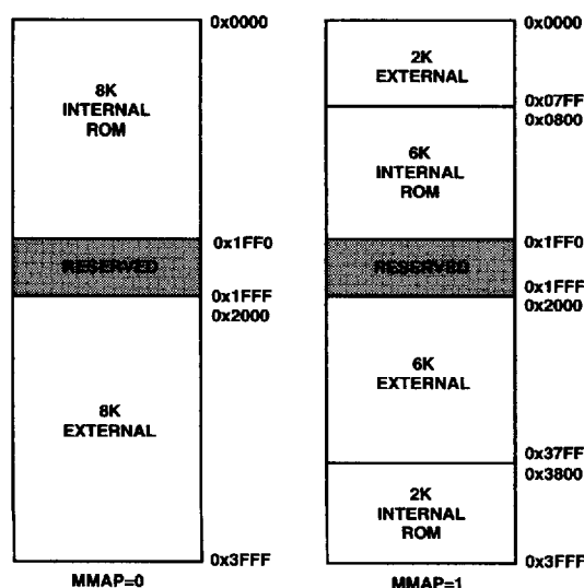
Figure 7. ADSP-2161/62 Program Memory Maps
