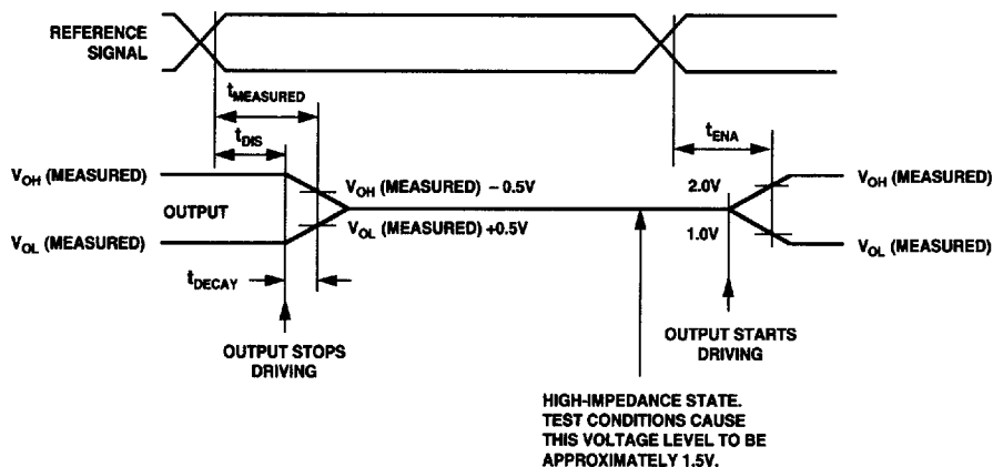
Figure 15. Output Enable/Disable
