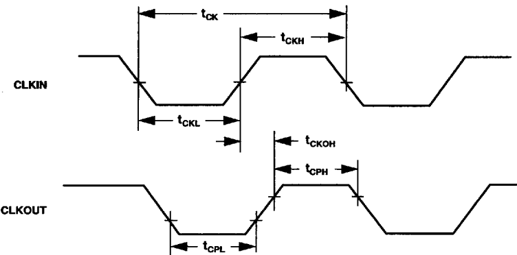
Figure 29. Clock Signals
