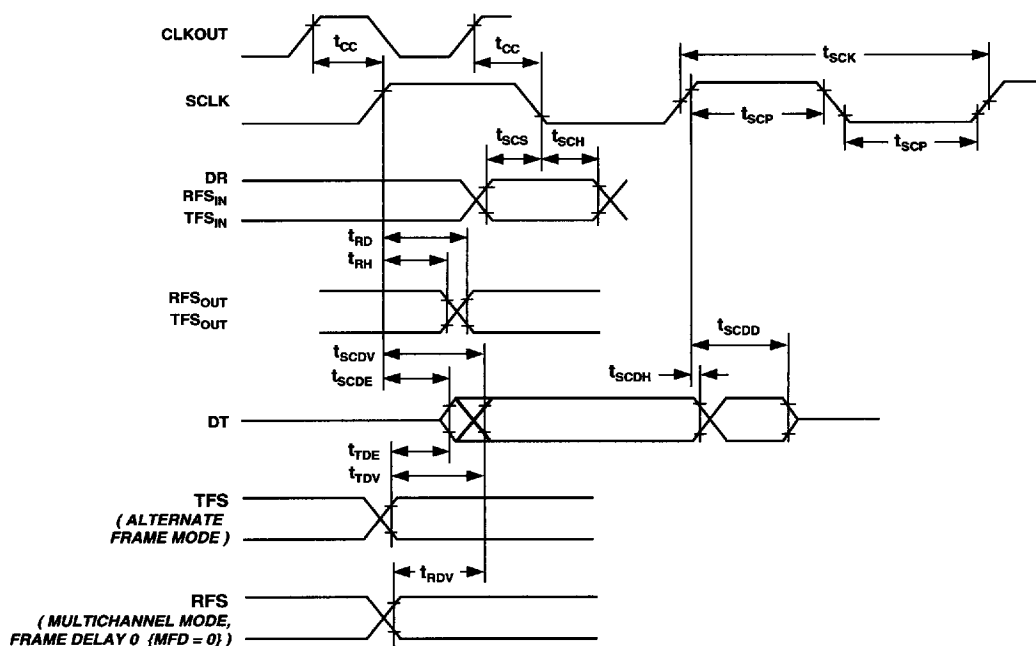
Figure 44. Serial Ports
