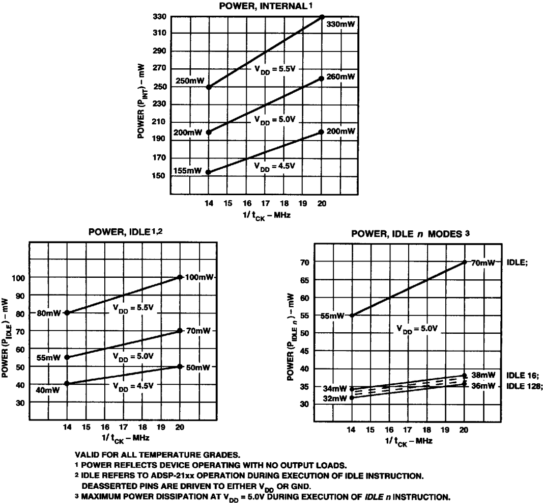
Figure 17. ADSP-2111 Power (Typical) vs. Frequency
