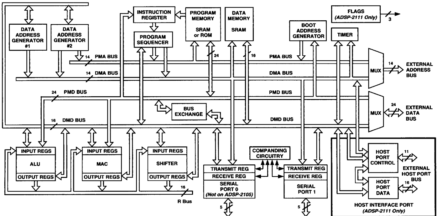
Figure 1. ADSP-21xx Block Diagram
