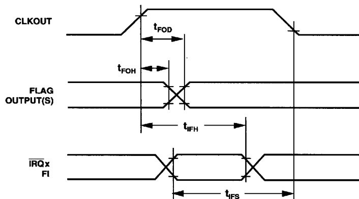
Figure 30. Interrupts &amp; Flags
