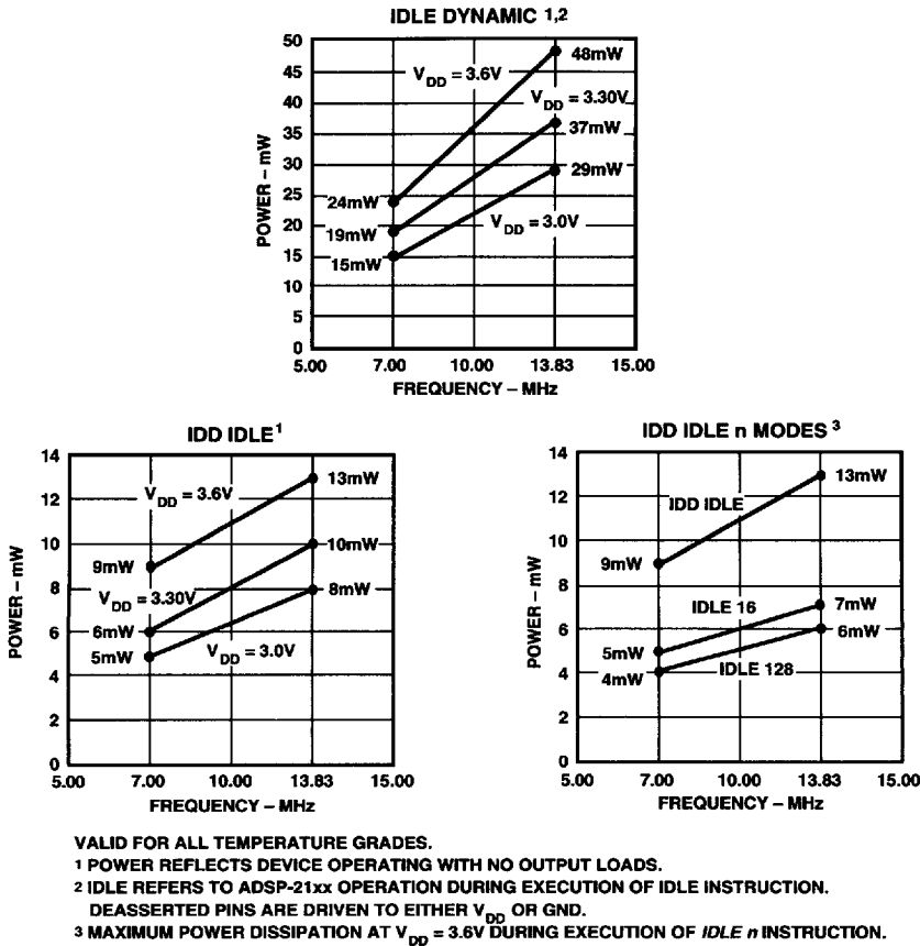
Figure 23. ADSP-2103 Power (Typical) vs. Frequency
