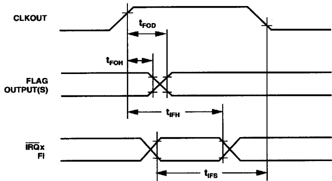
Figure 40. Interrupts & Flags
