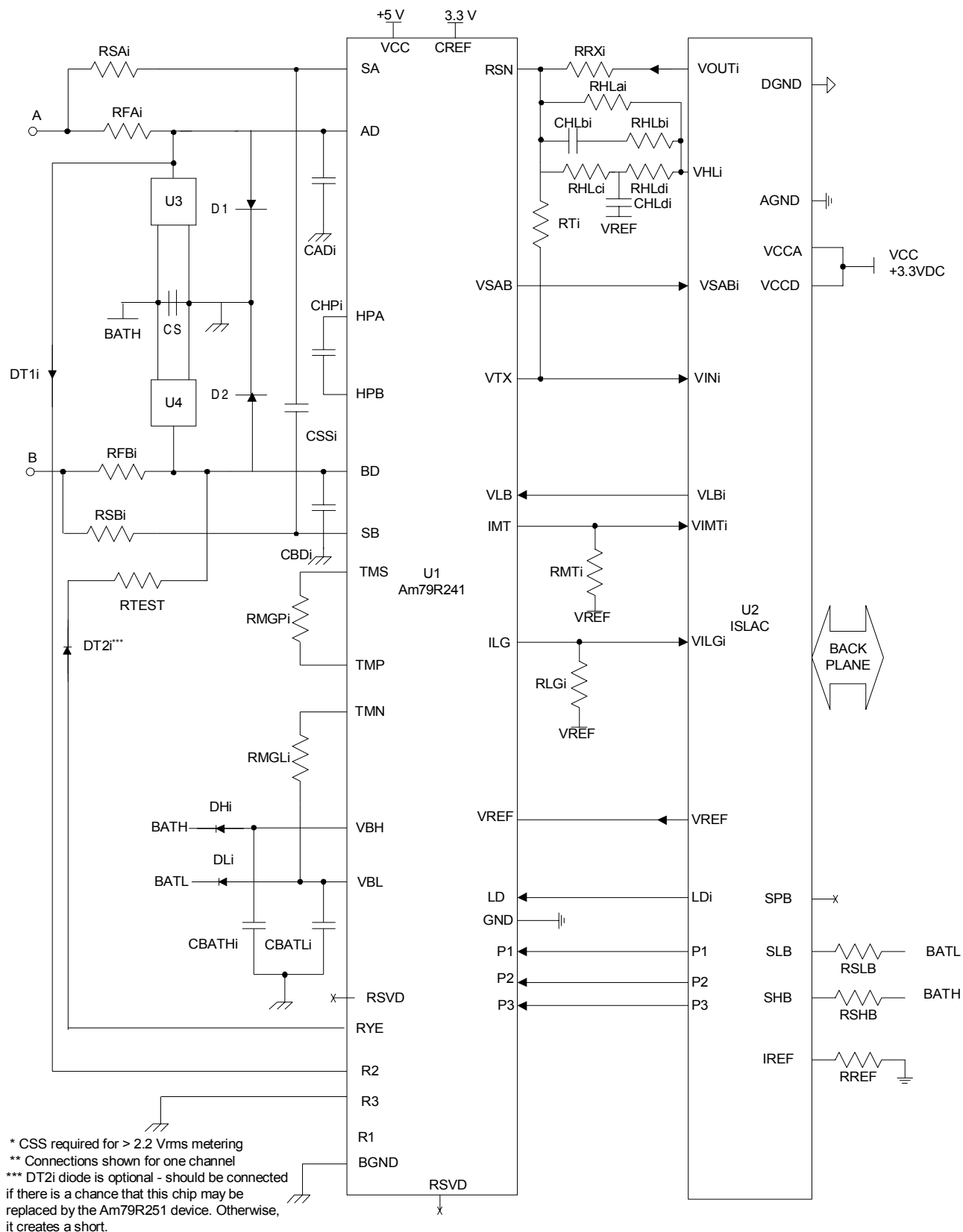
Figure 3. Internal Ringing Linecard Schematic
