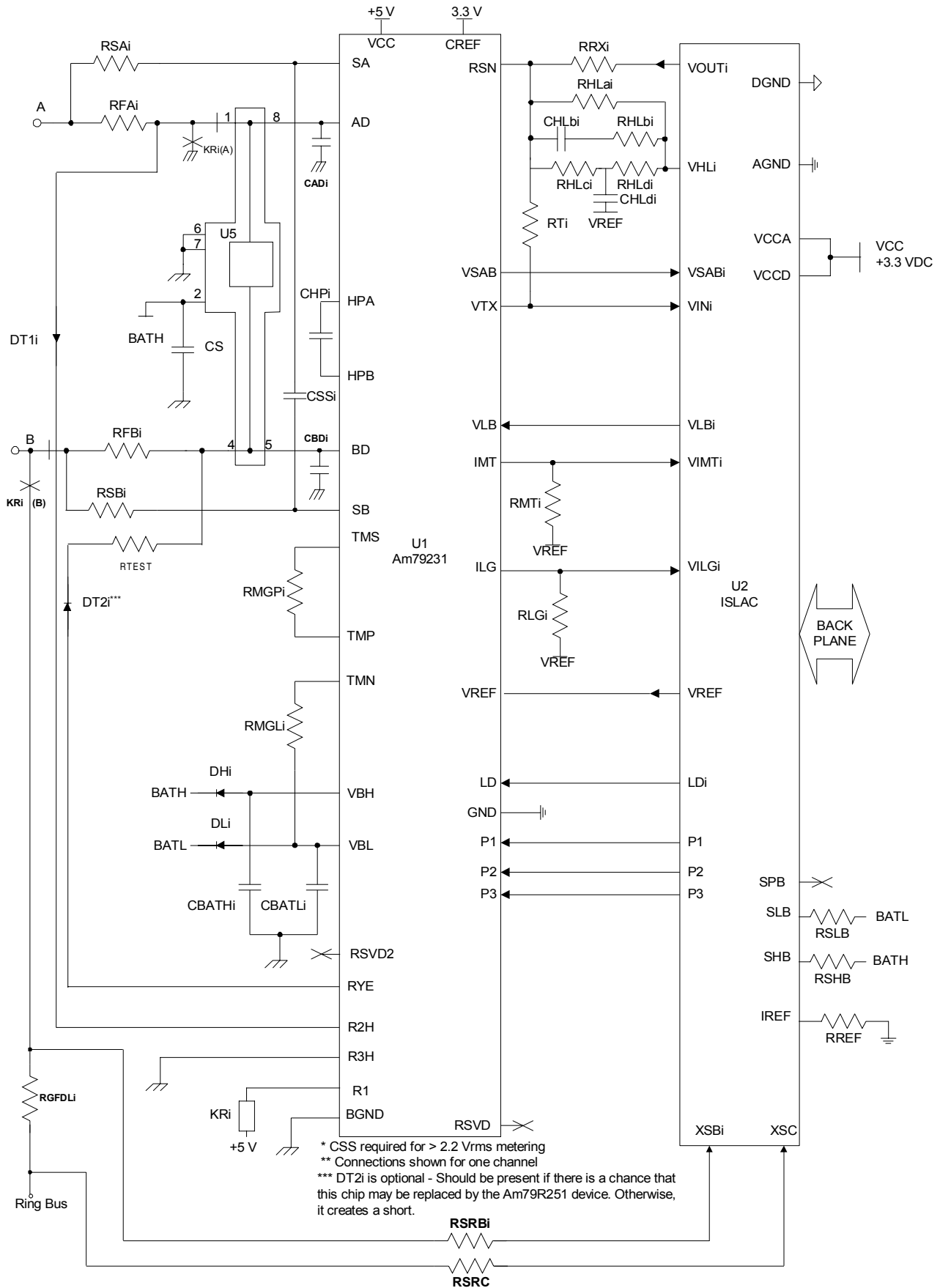
Figure 4. External Ringing Linecard Schematic
