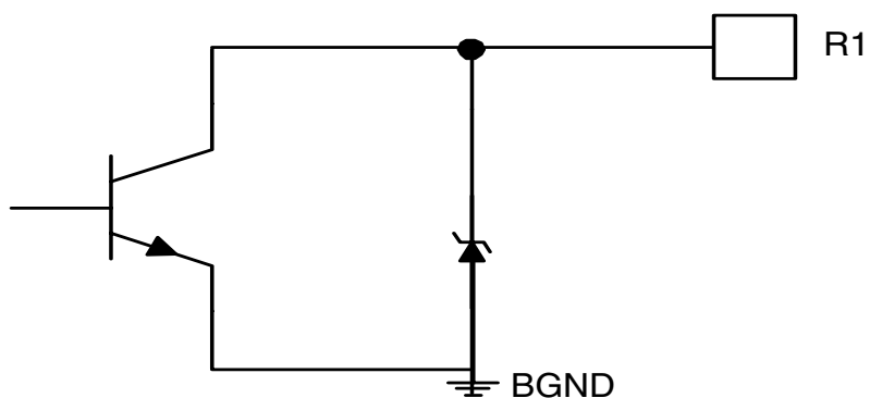
Figure 5A. Relay 1 Driver
