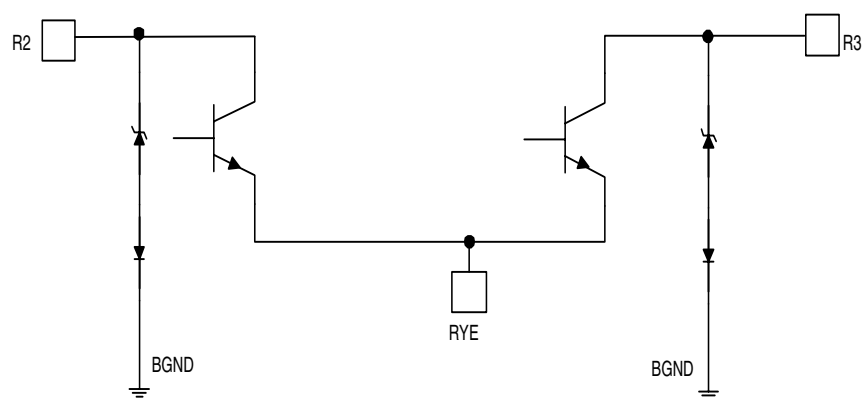
Figure 5. Relay Driver Configuration
