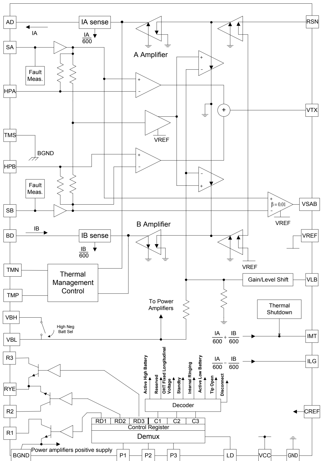
Figure 2. Am79R241 Block Diagram
