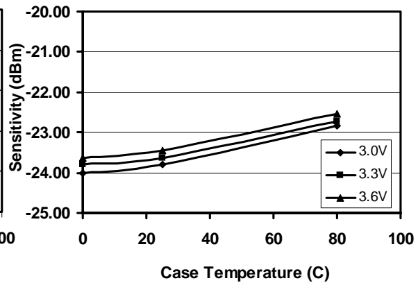
Figure 9: Sensitivity vs. Temperature
