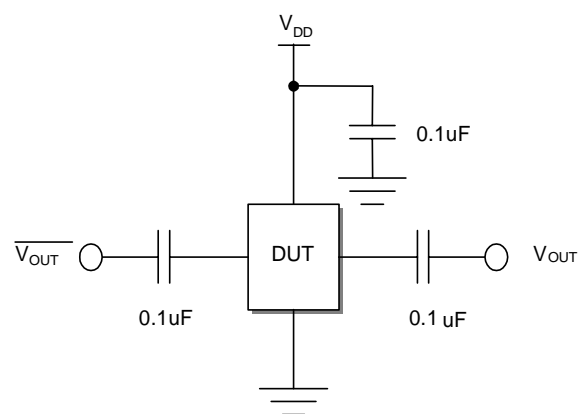
Figure 3: DUT Test Fixture Schematic
