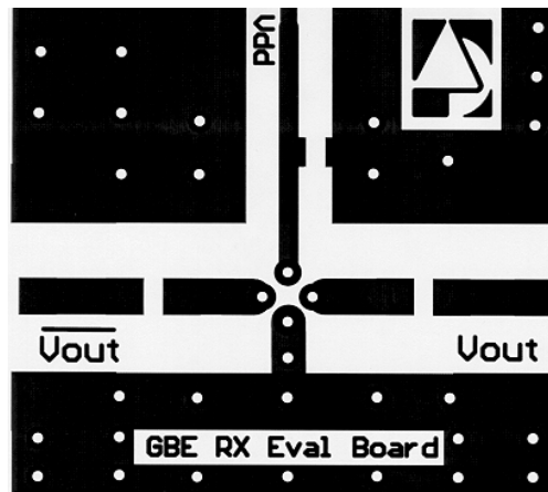
Figure 15: Evaluation Board Layout
