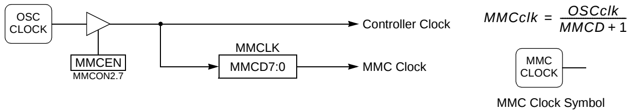
Figure 79. MMC Clock Generator and Symbol
