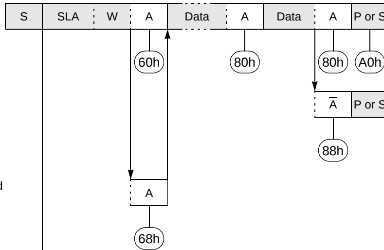
Figure 127. Format and States in the Slave Receiver Mode
