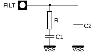
Figure 140. PLL Filter Connection
