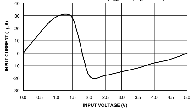
INPUT CURRENT VS. INPUT VOLTAGE (VCC = 5V, TA = 25°C)
