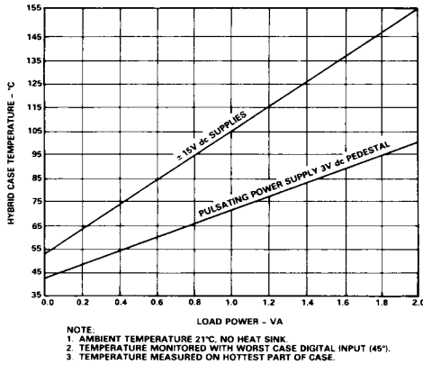
Figure 4. Case Temperature for Resistive Loads
