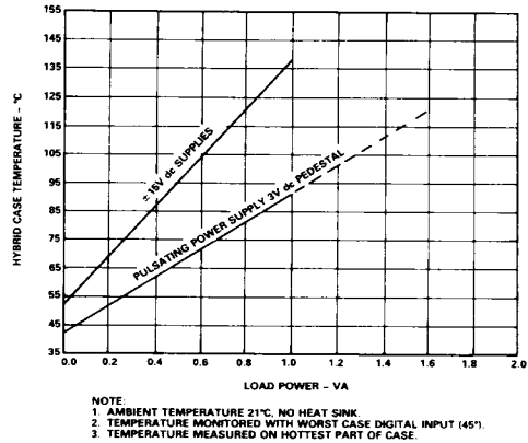
Figure 5. Case Temperature for Inductive Loads
