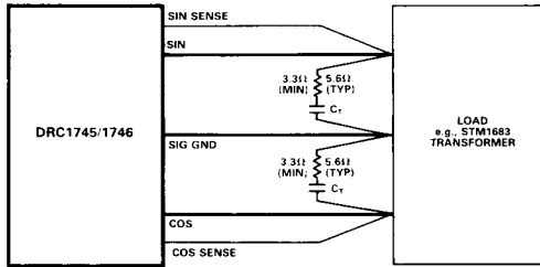
Figure 6. Incorporating a Resistor in the Tuning Circuit
