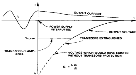
Figure 9. Transient Waveforms and TransZorb Clamping
