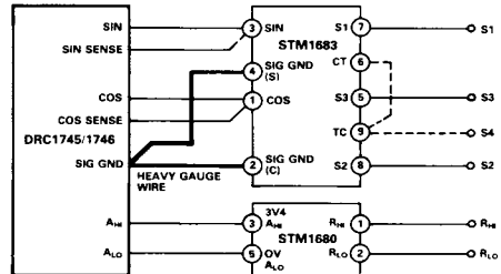
NOTE: FOR SYNCHRO OUTPUT "CT" MUST BE CONNECTED TO "TC" FOR RESOLVER OUTPUT "TC" IS S4 (NO LINK)
