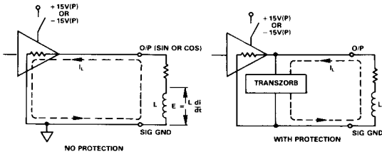
Figure 8. DRC1745/DRC1746 Output Stage Showing TransZorb Protection
