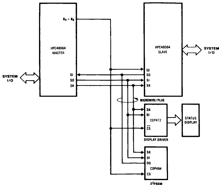
FIGURE 25. MICROWIRE/PLUS Application
