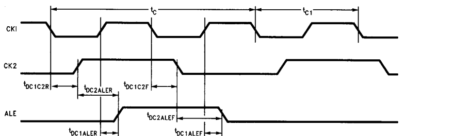
FIGURE 3. CKI, CK2, ALE Timing Diagram
