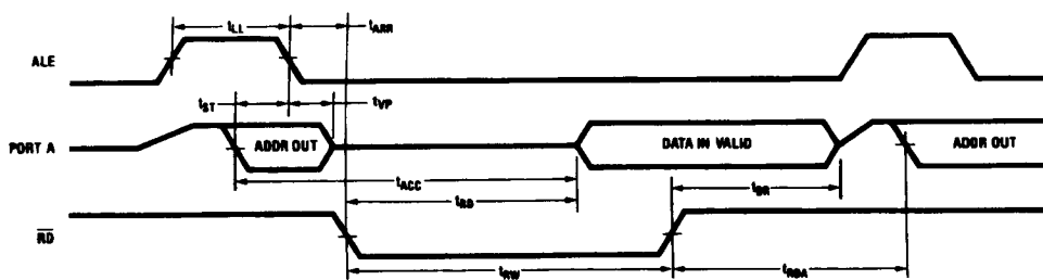
FIGURE 5. Read Cycle
