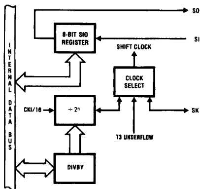
FIGURE 24. MICROWIRE/PLUS
