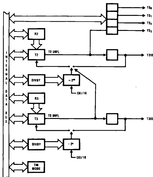
FIGURE 20. Timers T2-T3 Block
