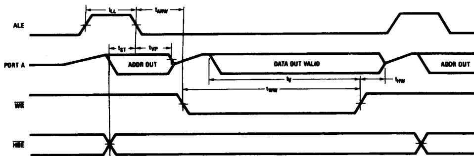
FIGURE 4. Write Cycle
