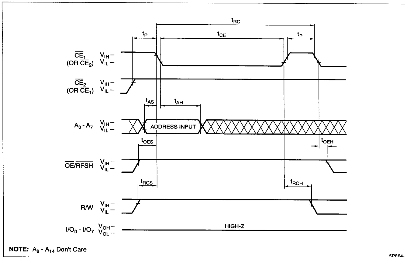
Figure 6. \overline{CE} Only Refresh Cycle
