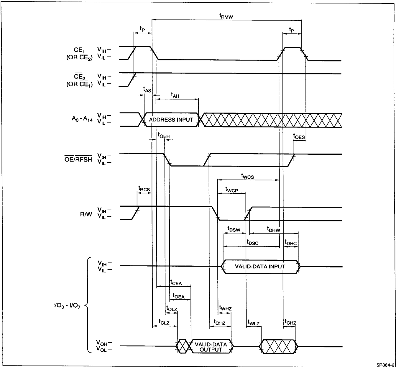
Figure 5. Read-Modify-Write Cycle
