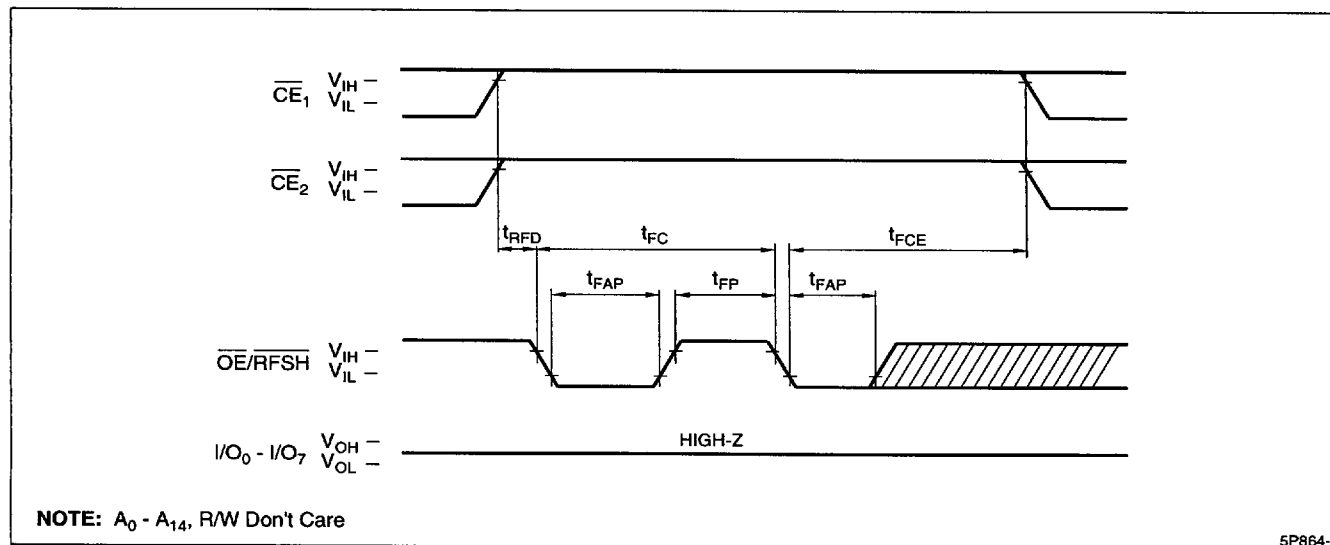
Figure 7. Auto Refresh Cycle
