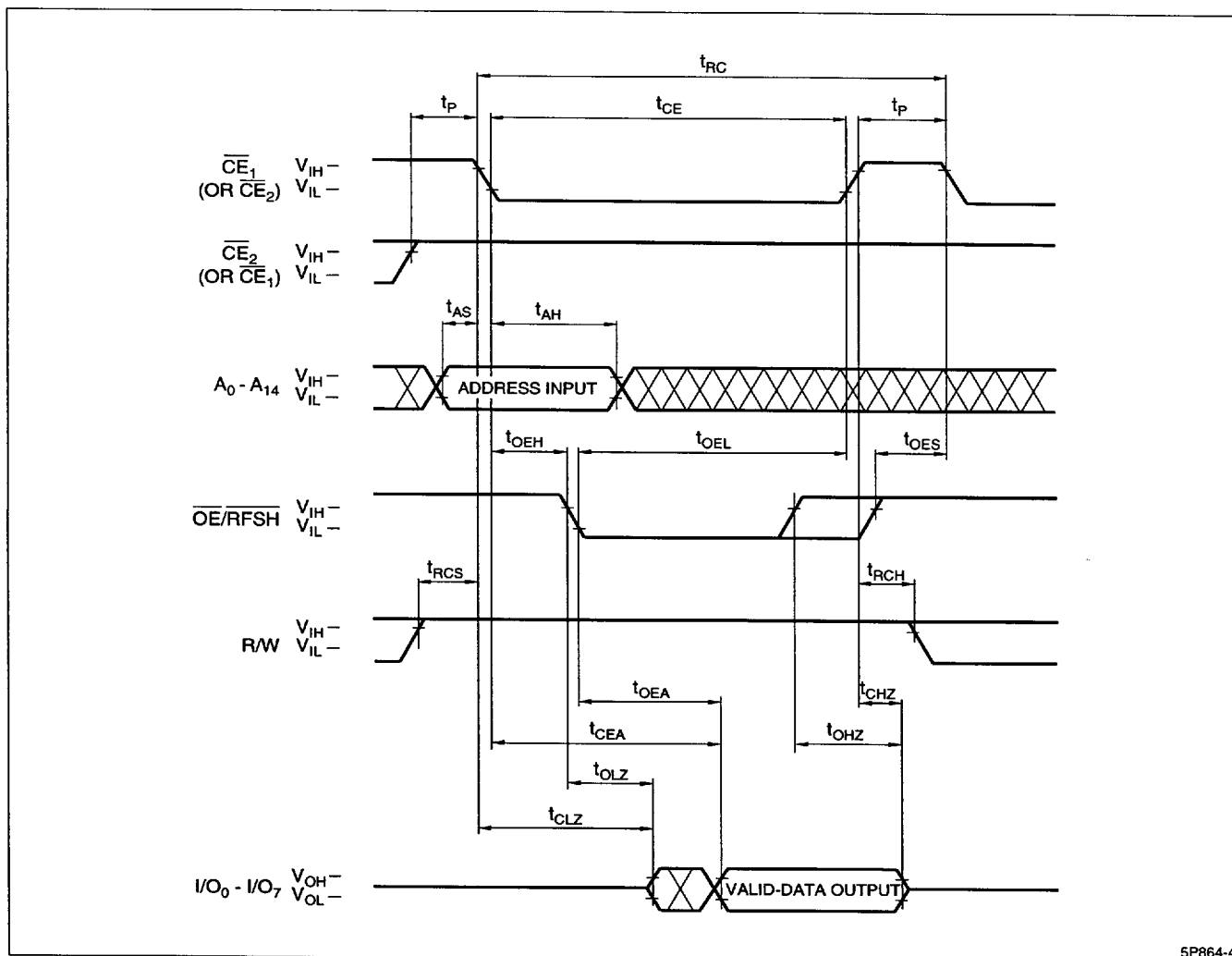
Figure 3. Read Cycle
