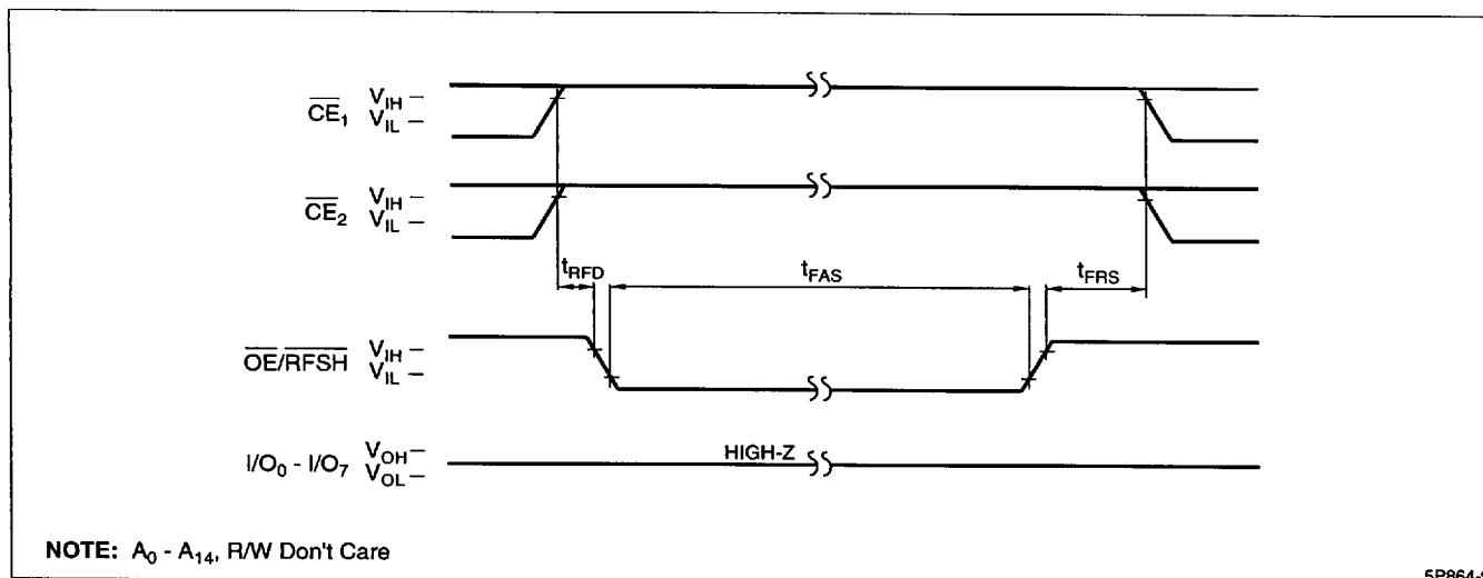
Figure 8. Self Refresh Cycle
