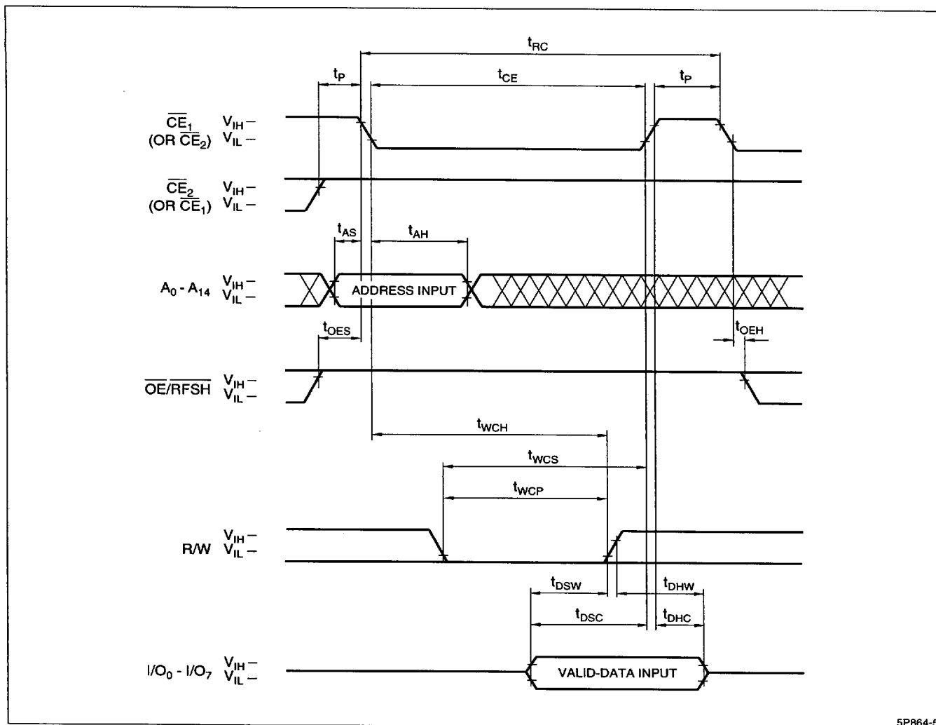
Figure 4. Write Cycle
