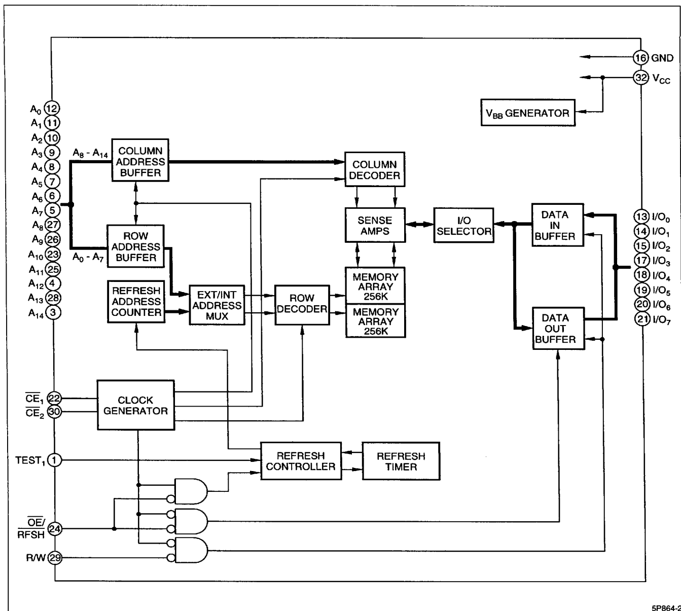
Figure 2. LH5P864 Block Diagram
