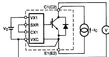
Figure 2 V_{EC} Test
