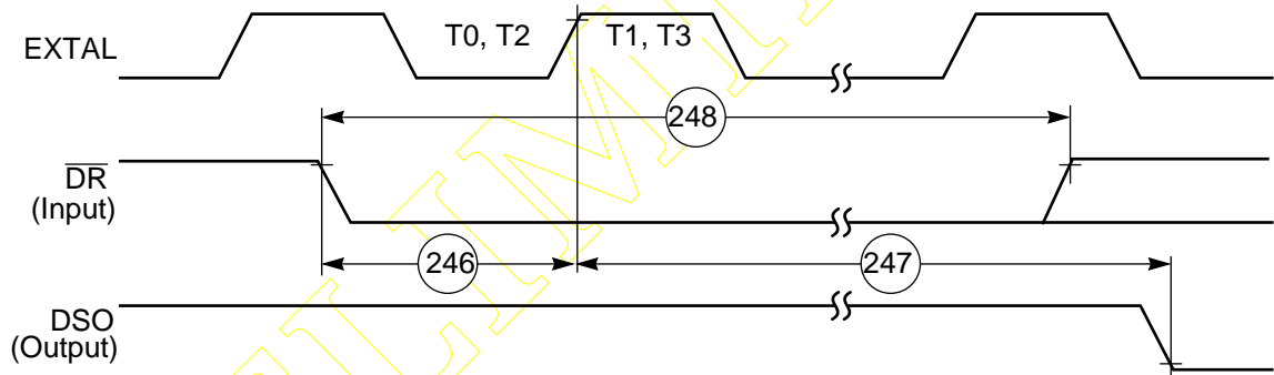
Figure 2-29 Synchronous Recovery from Wait State
