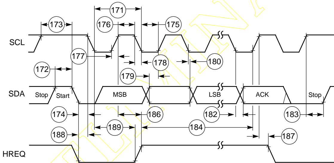
Figure 2-19 I 2 C Timing
