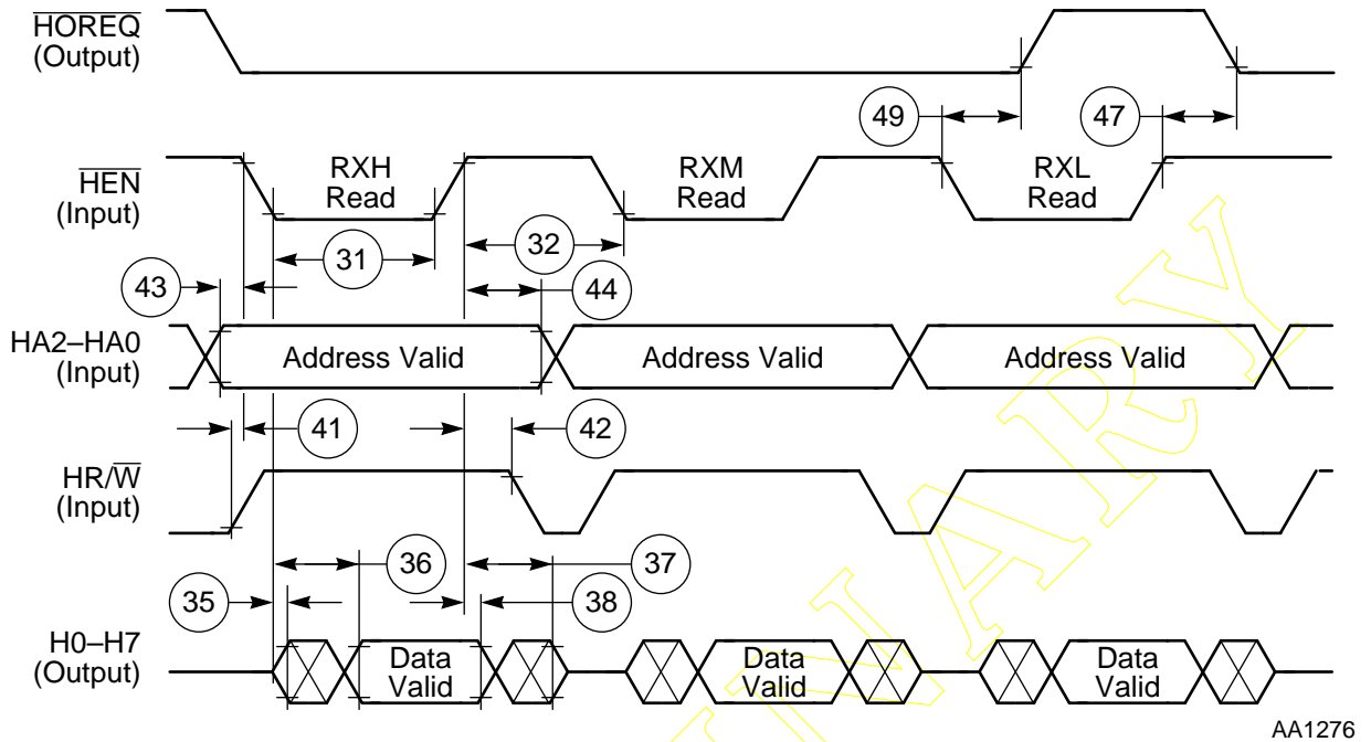
Figure 2-9 Host Read Cycle (Non-DMA Mode)
