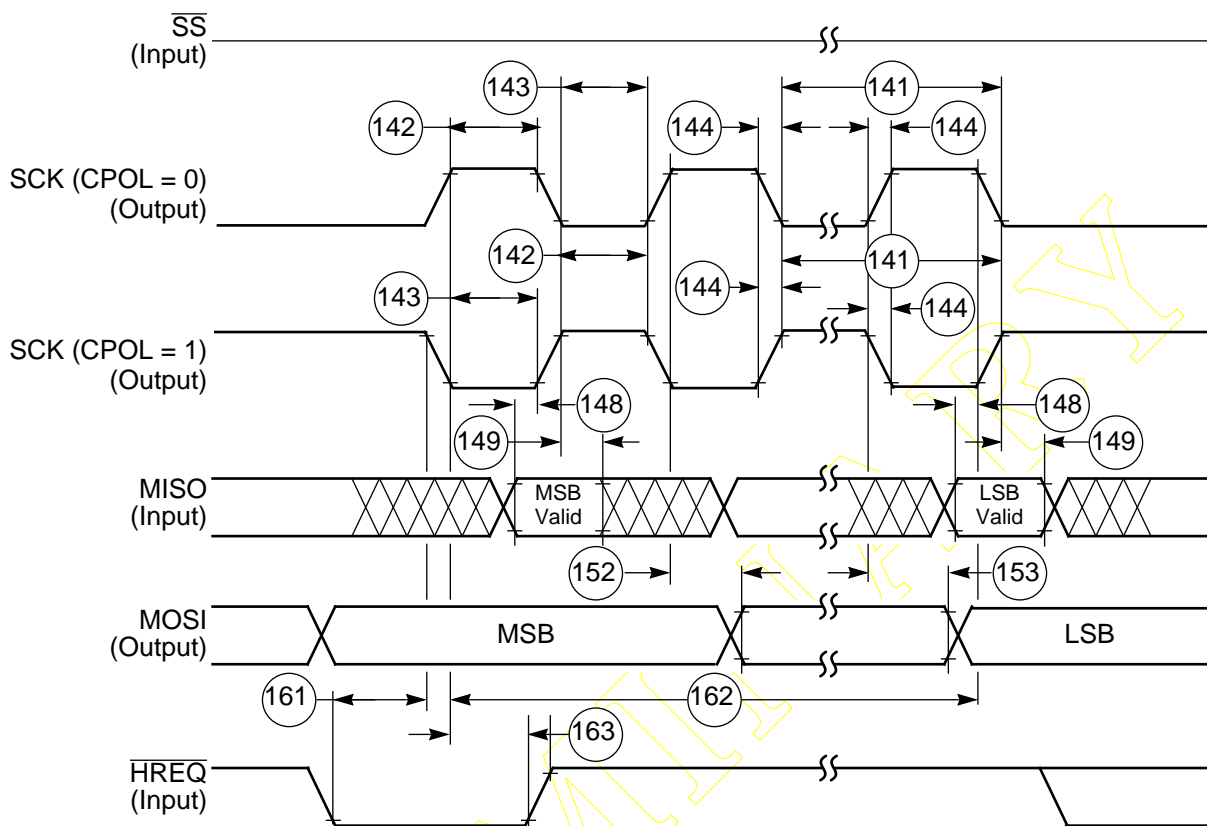
Figure 2-16 SPI Master Timing (CPHA = 1)
