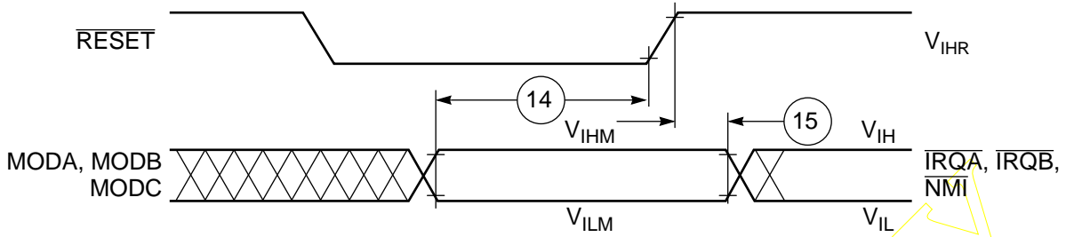
Figure 2-3 Operating Mode Select Timing
