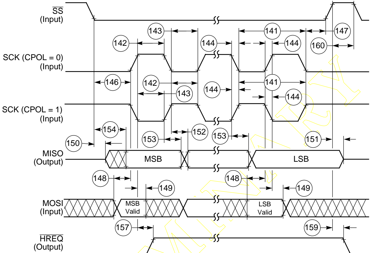
Figure 2-17 SPI Slave Timing (CPHA = 0)
