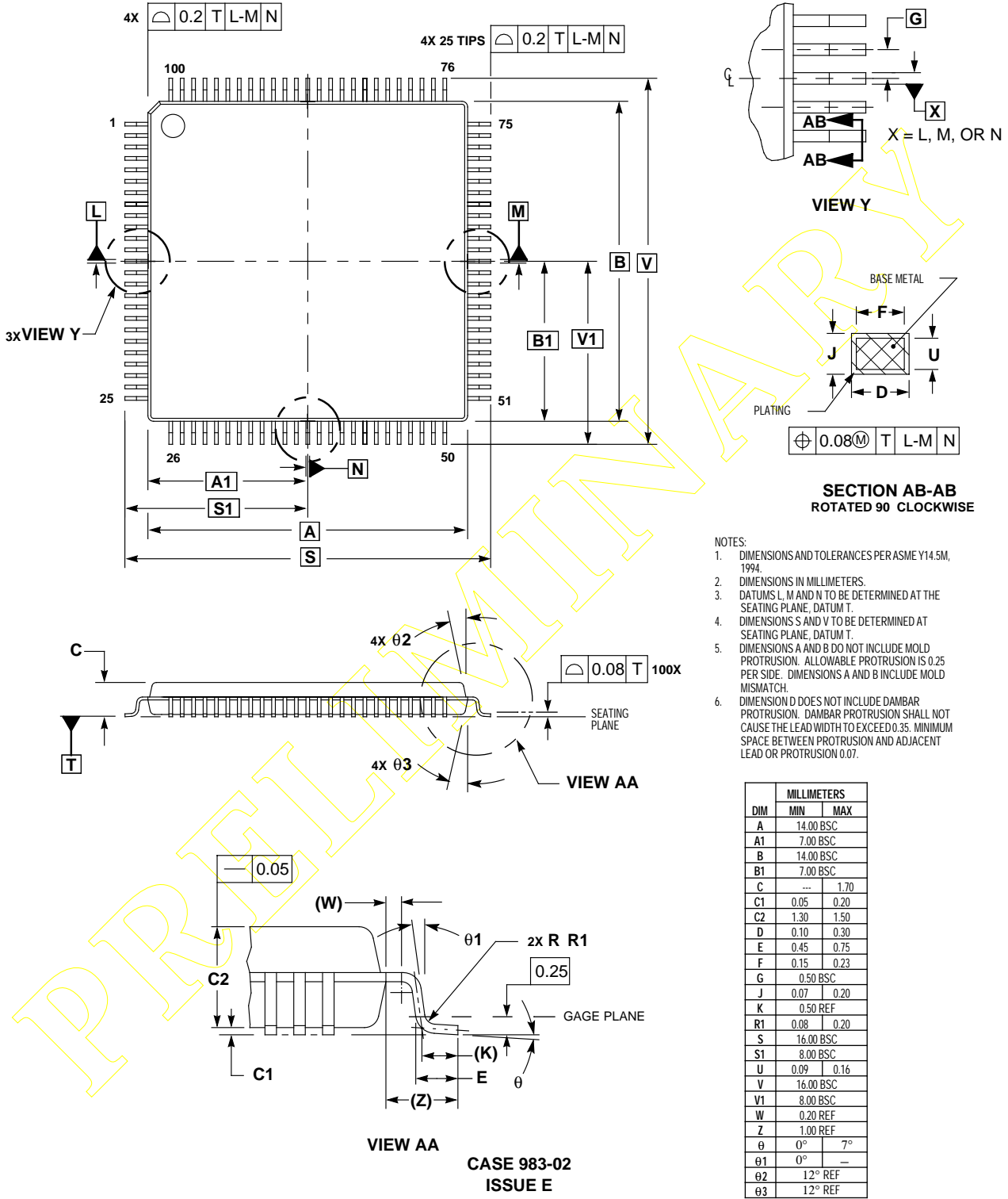
Figure 3-3 100-pin Thin Quad Flat Pack (TQFP) Mechanical Information
