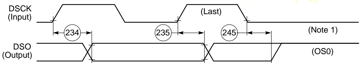
Figure 2-24 DSP56011 OnCE Data I/O to Status Timing
