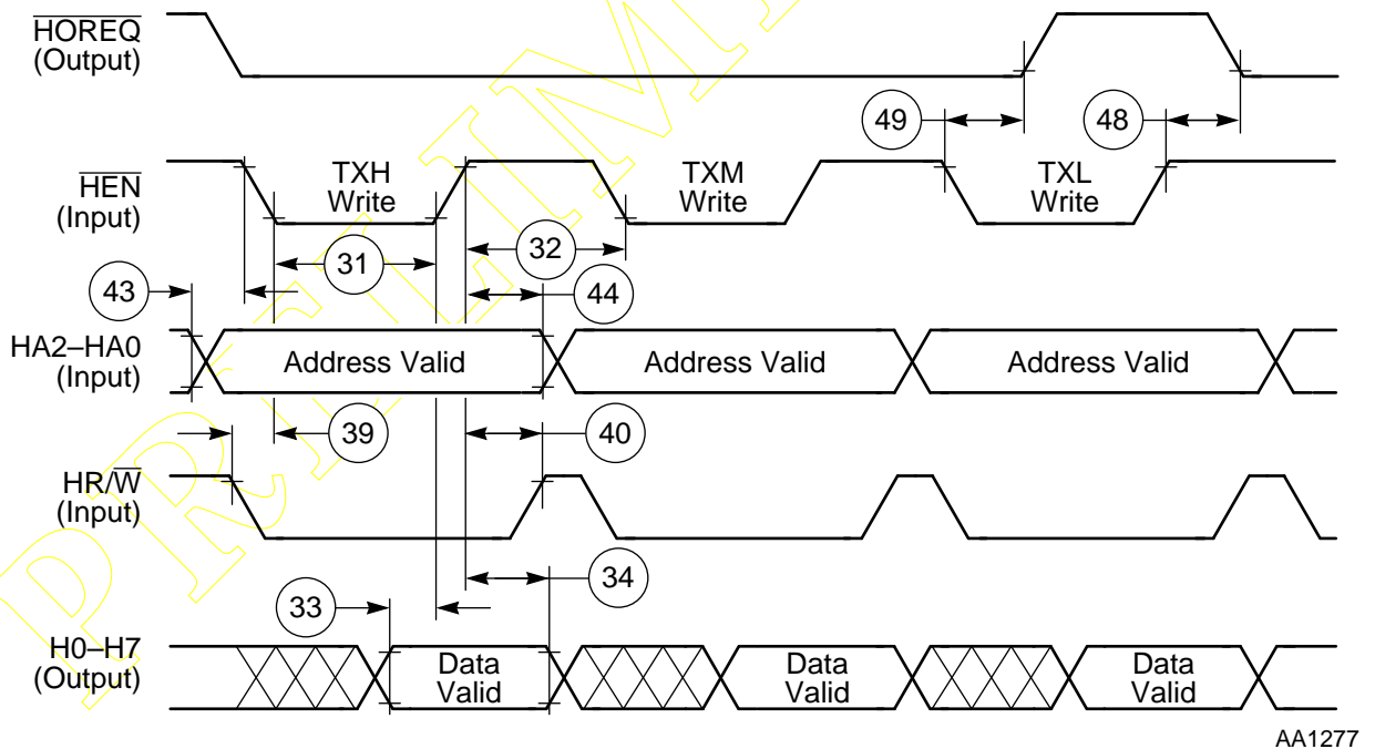
Figure 2-10 Host Write Cycle (Non-DMA Mode)
