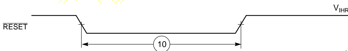
Figure 2-2 Reset Timing
