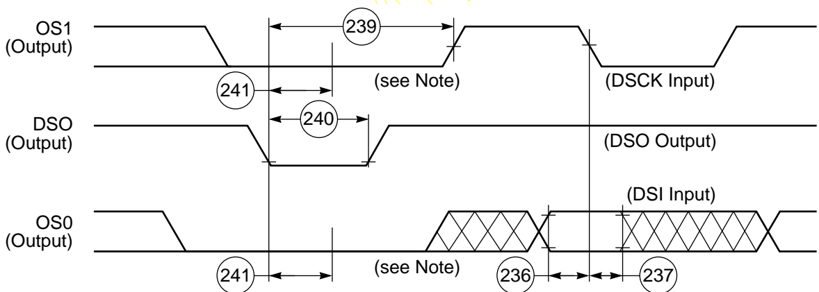
Figure 2-25 DSP56011 OnCE Read Timing
