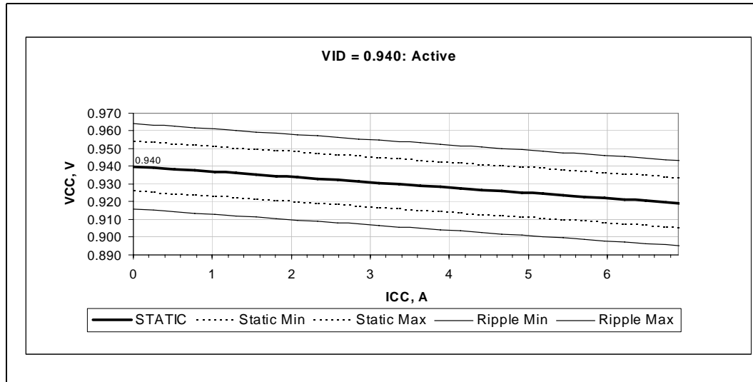
Figure 3. Illustration of Active State V_{CC} Static and Ripple Tolerances for the Celeron M Processor ULV: VID=0.940 V
