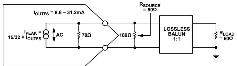
Figure 96. Equivalent Circuit for Determining Maximum Peak Power to a 50\ \Omega Load
