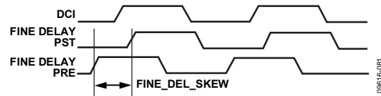
Figure 78. Pre- and Post-Delay Sampling Diagram
