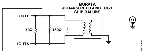
Figure 101. Lowest Cost and Size Configuration for Narrow RF Band Operation
