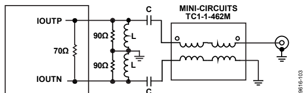
Figure 100. Recommended Mix-Mode Configuration Offering Extended RF Bandwidth Using a TC1-1-462M Balun
