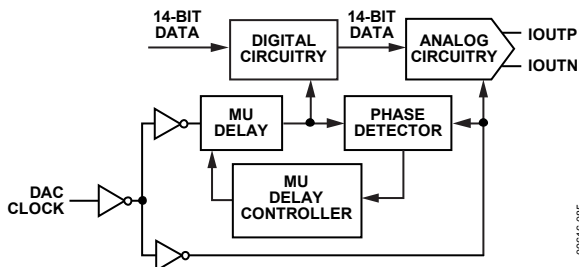
Figure 82. Mu Delay Controller Block Diagram
