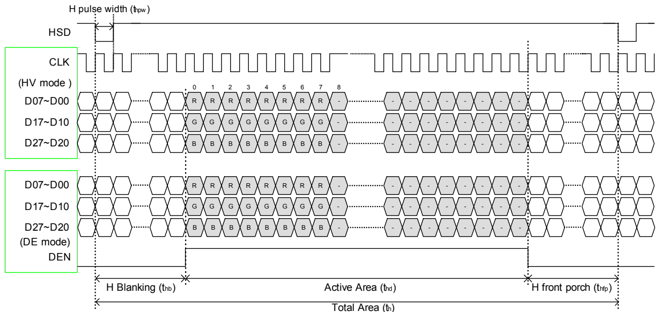
Horizontal display timing range
