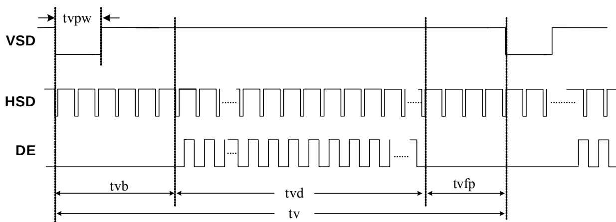
Vertical timing
