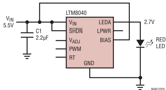
Figure 2b. BIAS May be Tied to XV_{IN} if LPWR is Below 2.6V
