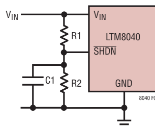
Figure 1. Undervoltage Lockout
