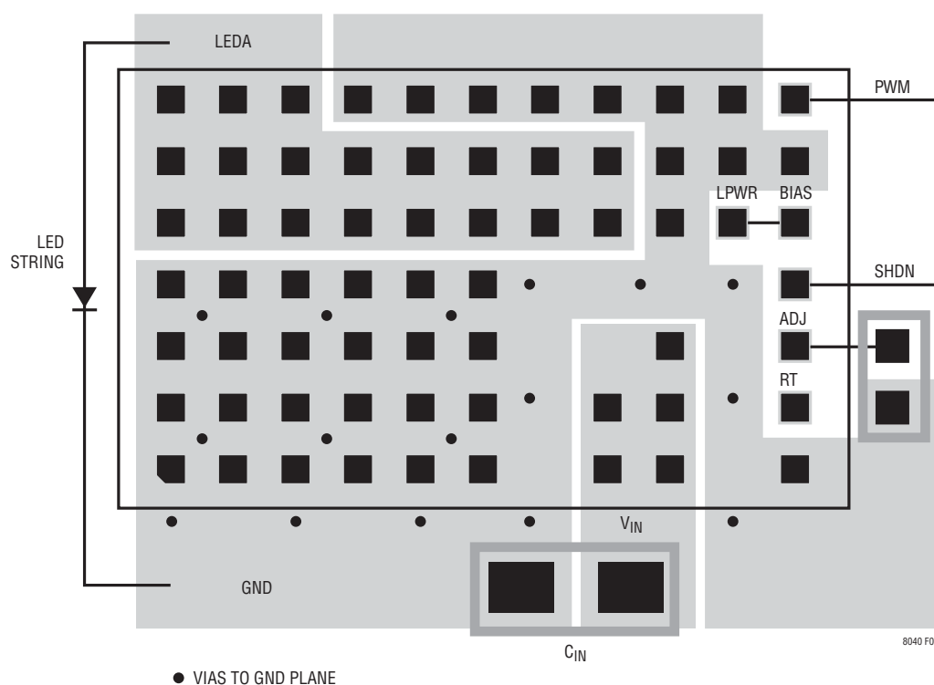
Figure 6. Suggested Layout
