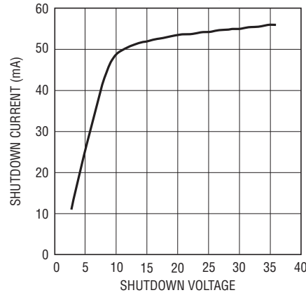
\overline{SHDN} Current vs Voltage
