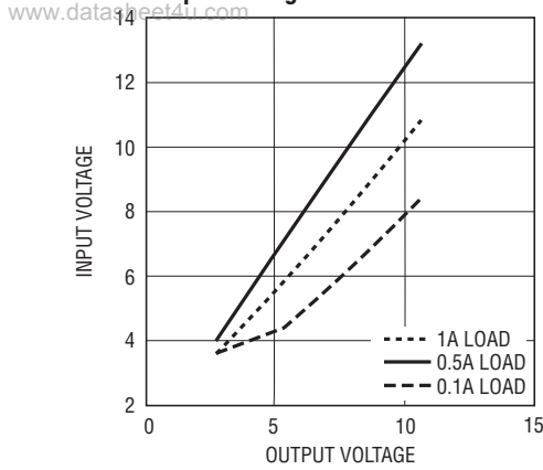
Minimum Running Voltage vs Output Voltage 2.7V at 1A LEDs
