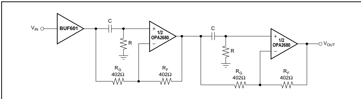
FIGURE 7. Two Stage, All-Pass Network.
