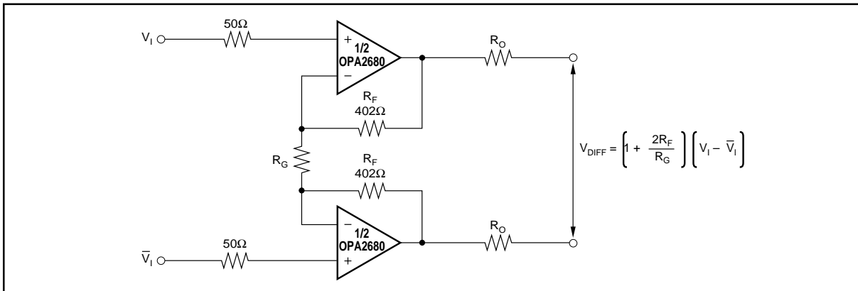
FIGURE 8. High Speed Differential Receiver.
