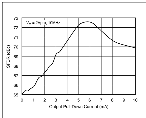
FIGURE 4. SFDR vs I_B .
