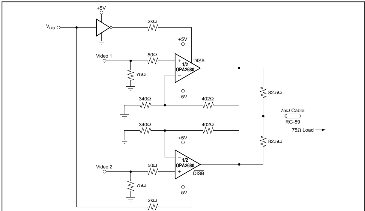
FIGURE 6. Two-Channel Video Multiplexer (SO-14 package only).
