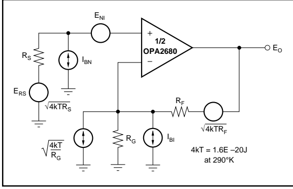
FIGURE 12. Op Amp Noise Analysis Model.
