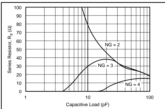
FIGURE 11. Required R_S vs Noise Gain.
