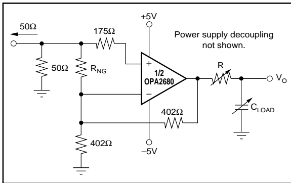
FIGURE 10. Capacitive Load Driving with Noise Gain Tuning.
