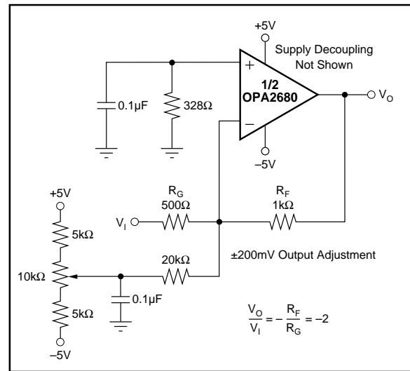
FIGURE 13. DC-Coupled, Inverting Gain of -2, with Offset Adjustment.
