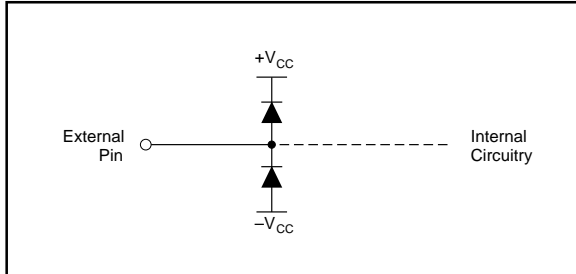
FIGURE 16. Internal ESD Protection.
