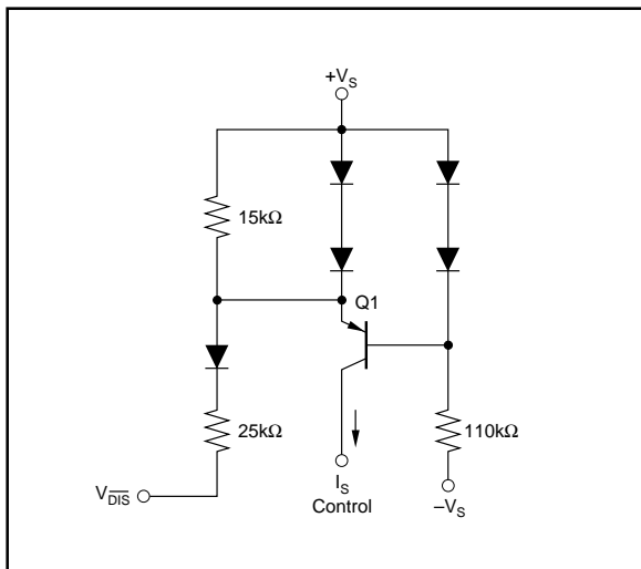
FIGURE 14. Simplified Disable Control Circuit.
