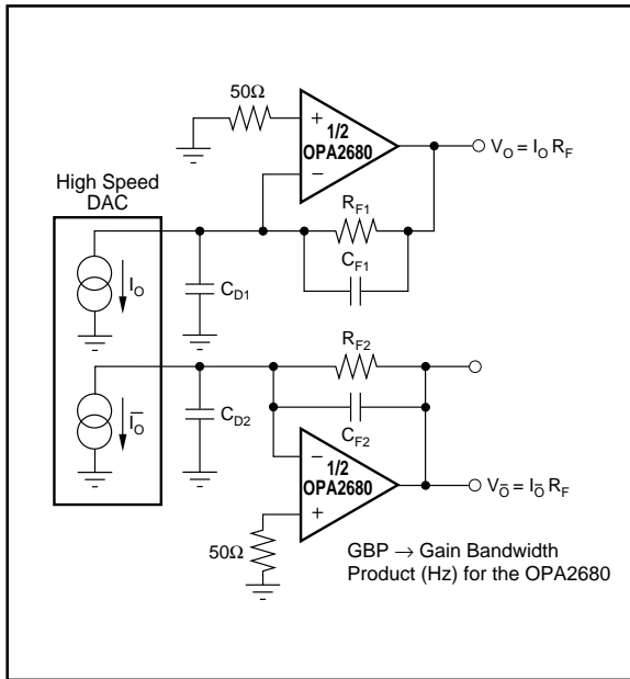
FIGURE 5. High Speed DAC—Differential Transimpedance Amplifier
