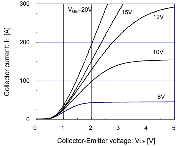
[ Inverter ] Collector current vs. Collector-Emittor voltage (typ.) T_j = 150^\circ\text{C} / \text{chip}
