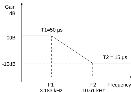
Figure 6. De-Emphasis Curve
