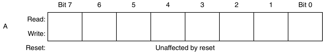
Figure 8-2. Accumulator (A)
