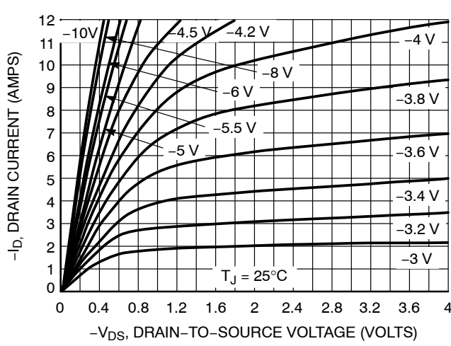
Figure 27. On-Region Characteristics
