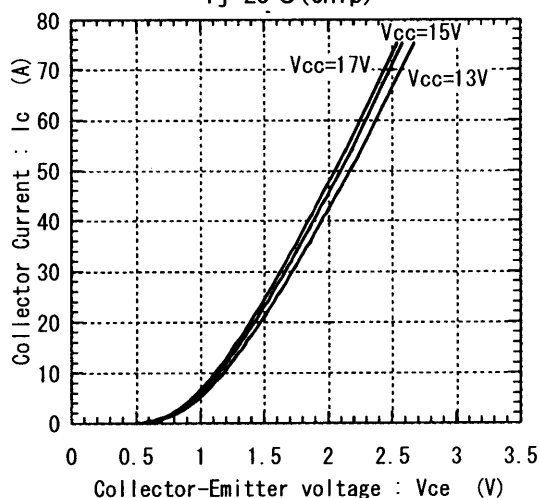
Collector current vs. Collector-Emitter voltage T_j=25^\circ\text{C} (Chip)
