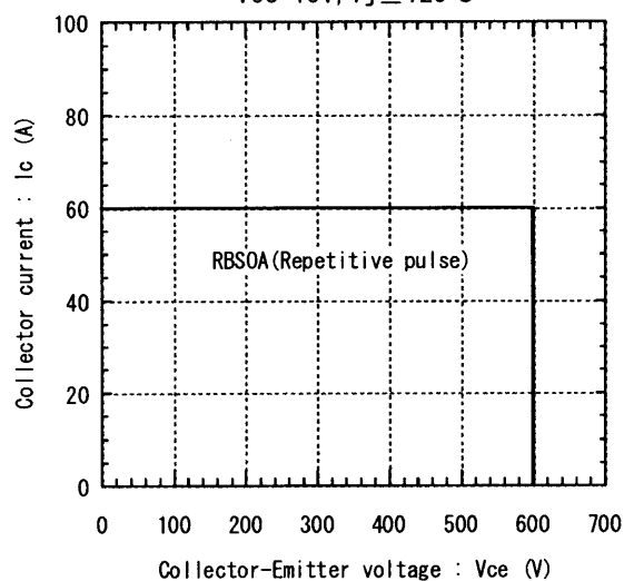
Reversed biased safe operating area V_{cc}=15\text{V} , T_j \leq 125^{\circ}\text{C}
