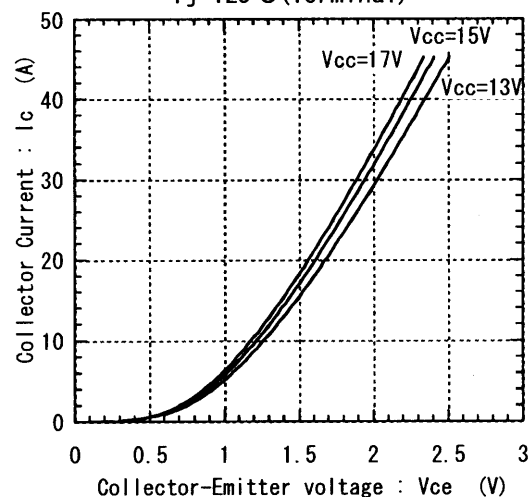
Collector current vs. Collector-Emitter voltage T_j=125^{\circ}\text{C} (Terminal)
