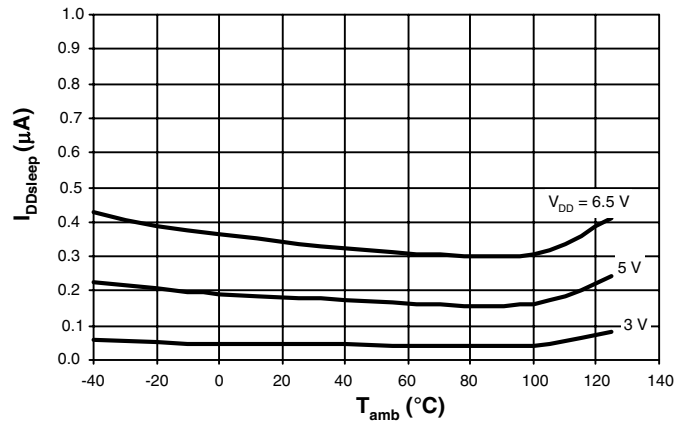
Figure 91. Sleep Current versus T_{amb}
