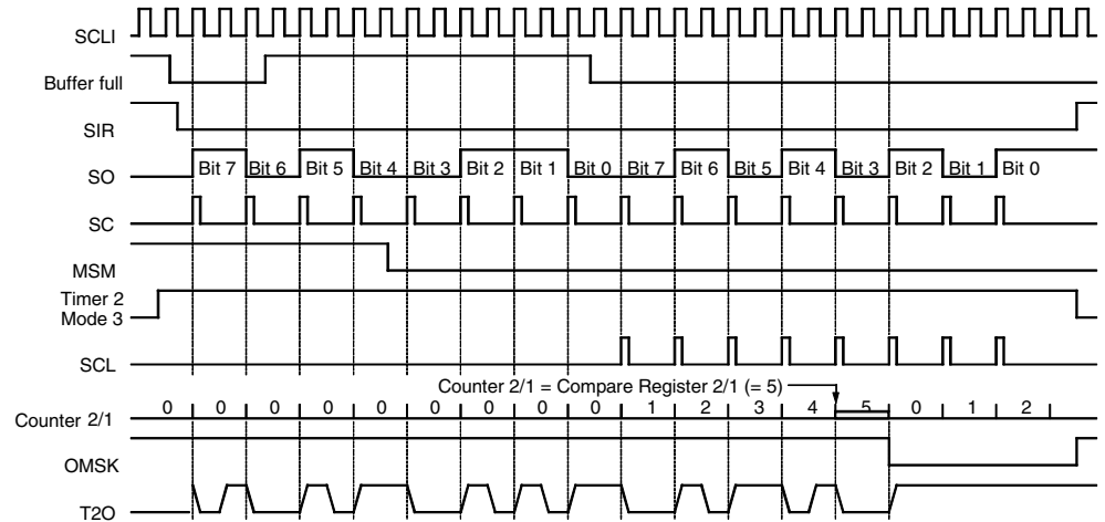
Figure 72. Bi-phase Modulation 2
