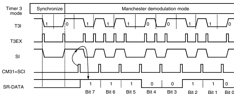
Figure 76. Manchester Demodulation
