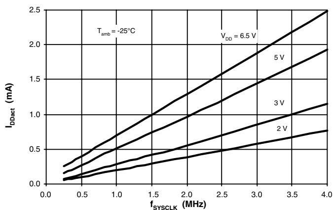
Figure 87. Active Supply Current versus Frequency
