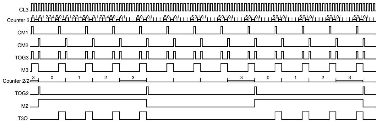
Figure 81. Burst Modulation 1
