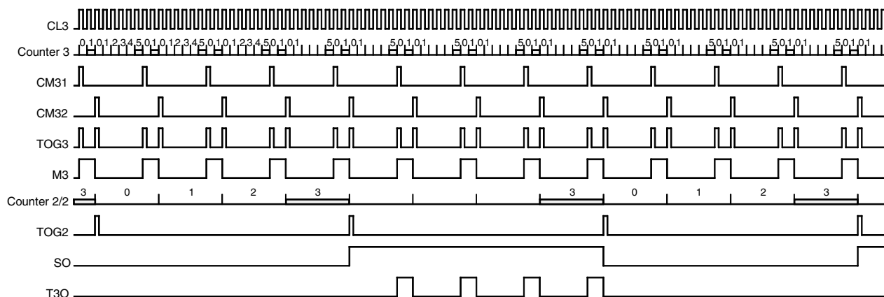
Figure 83. Burst Modulation 2
