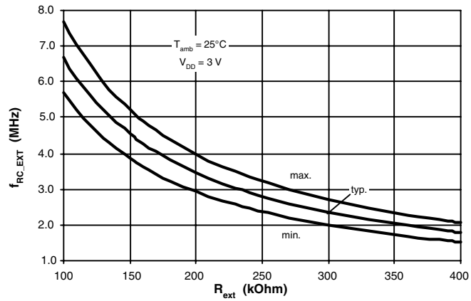
Figure 97. External RC Frequency versus R_{ext}
