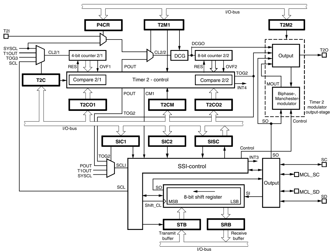
Figure 67. Combination Timer 2 and SSI
