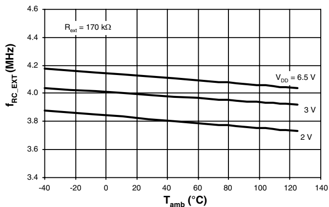
Figure 95. External RC Frequency versus T_{amb}
