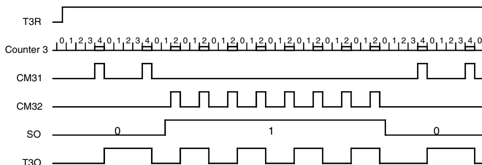
Figure 74. FSK Modulation 1
