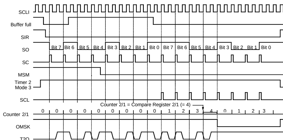
Figure 79. Manchester Modulation 2
