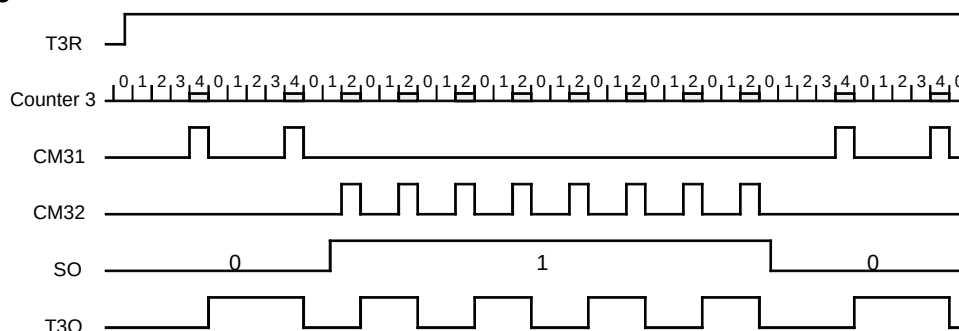
Figure 82. FSK Modulation
