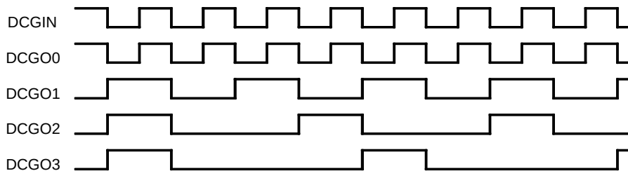
Figure 50. DCG Output Signals
