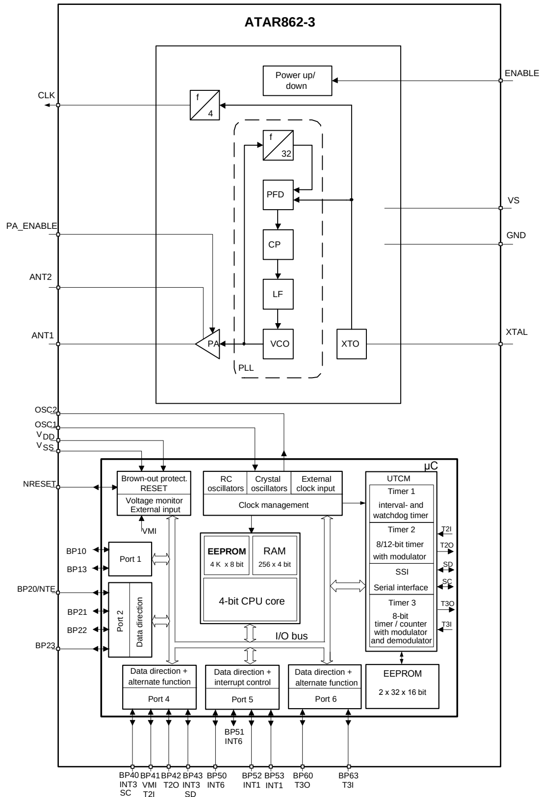
Figure 3. Block Diagram
