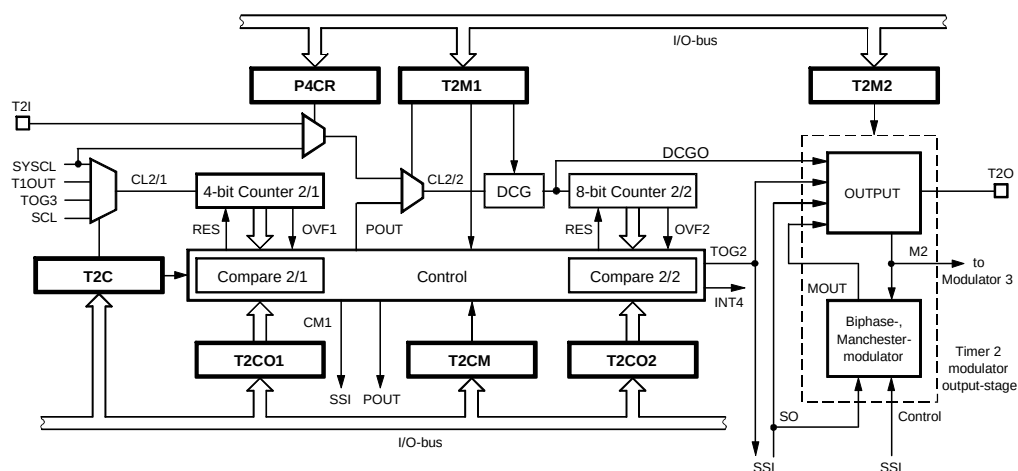
Figure 37. Timer 2
