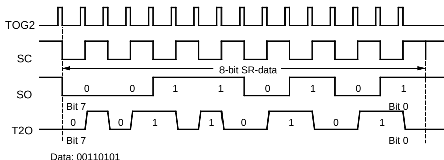
Figure 78. Manchester Modulation 1
