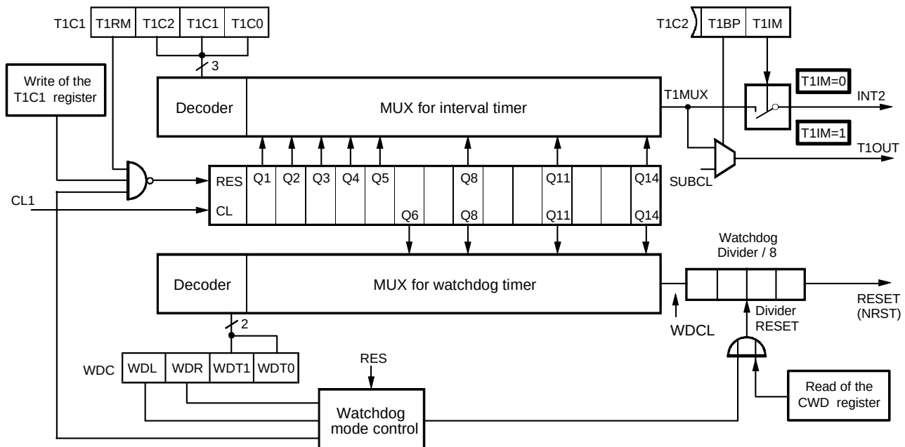
Figure 36. Timer 1 and Watchdog
