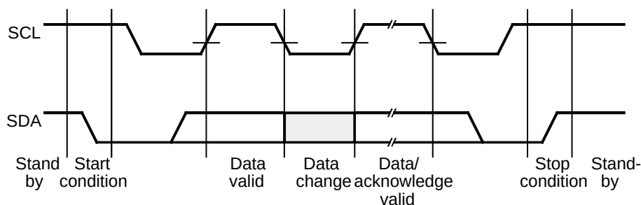
Figure 95. MCL Protocol
