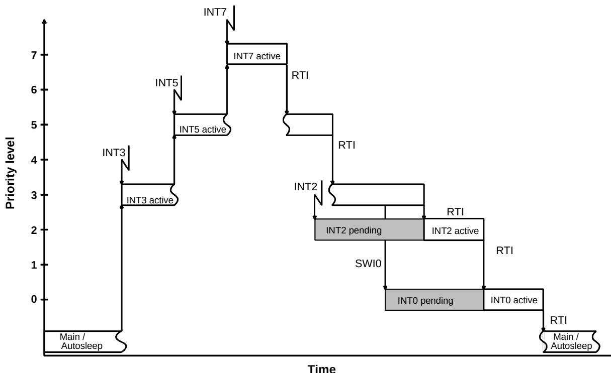
Figure 15. Interrupt Handling
