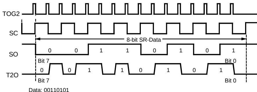
Figure 48. Manchester Modulation
