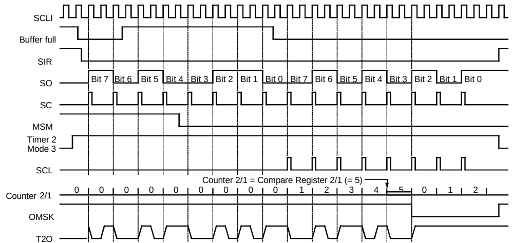
Figure 80. Biphase Modulation
