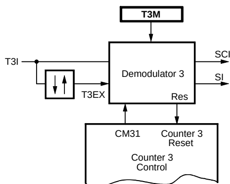
Figure 64. Timer 3 Demodulator 3
