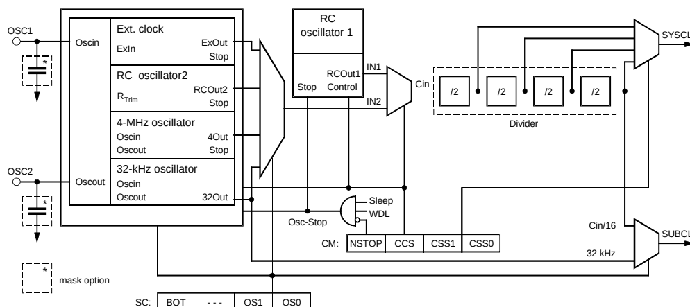
Figure 21. Clock Module
