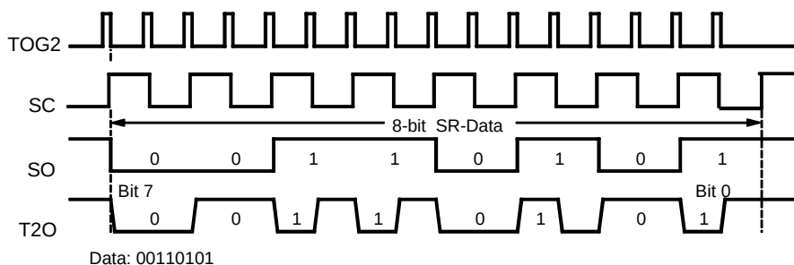
Figure 47. Biphase Modulation
