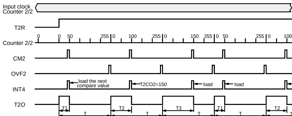
Figure 49. PWM Modulation
