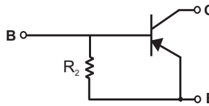
SCHEMATIC DIAGRAM
