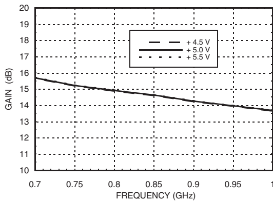
Gain vs. Vdd
