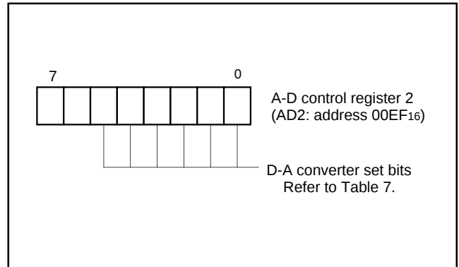
Fig. 29. Structure of A-D control register 2
