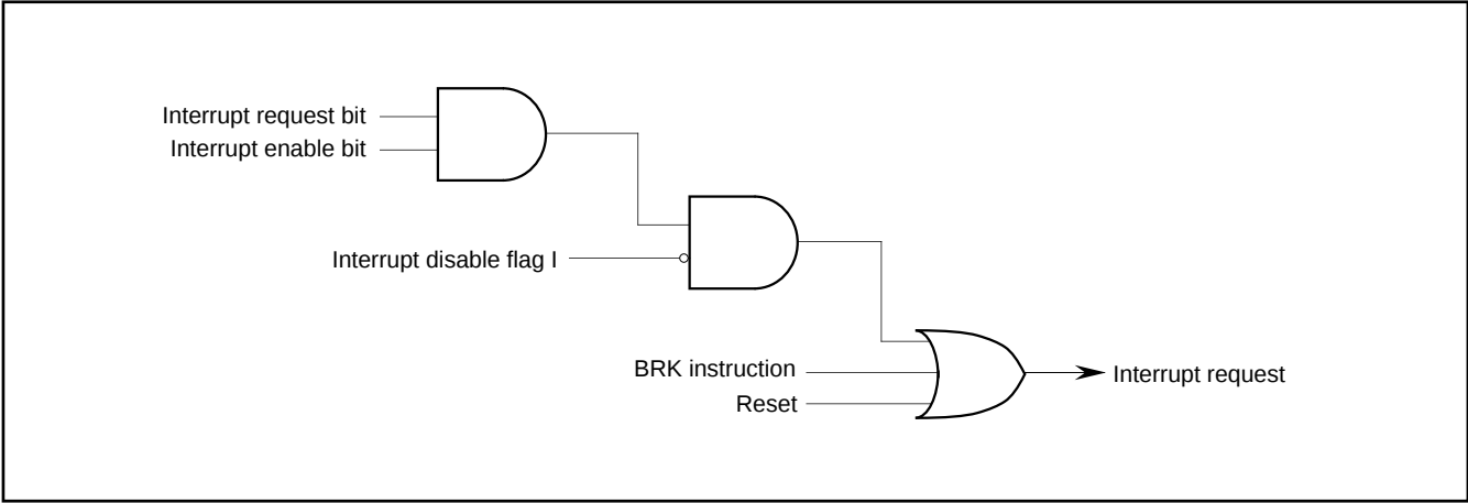
Fig. 5. Interrupt control
