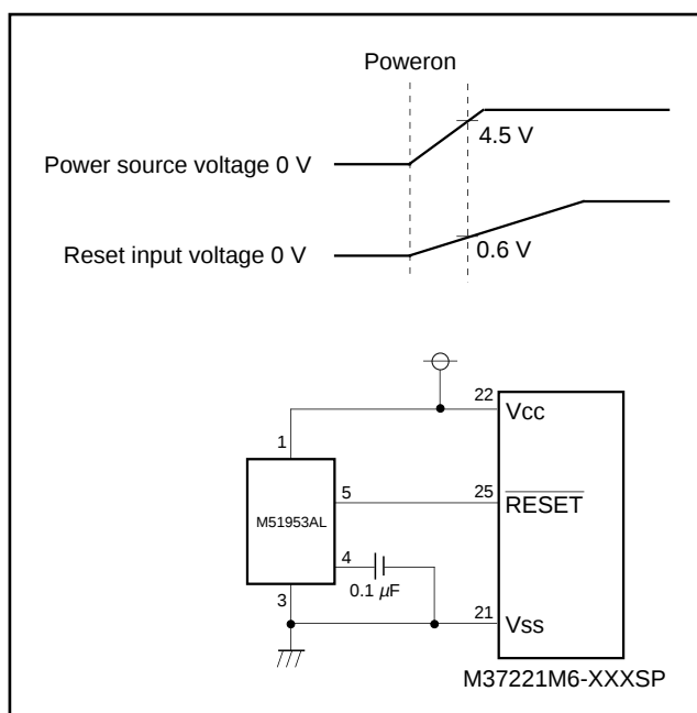
Fig. 50. Example of reset circuit
