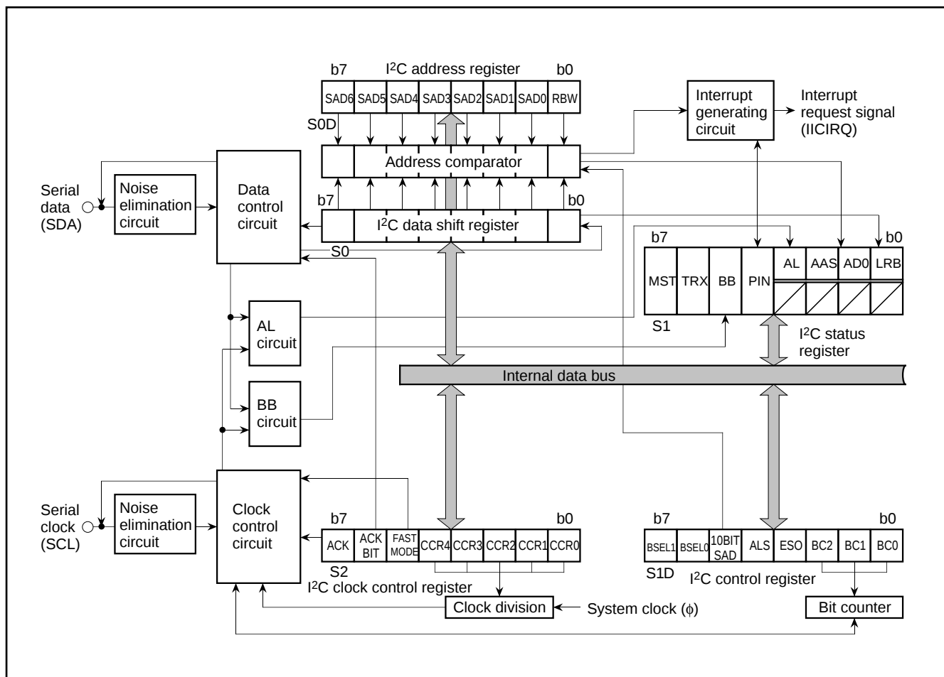
Fig. 12. Block diagram of multimaster I 2 C-BUS interface
