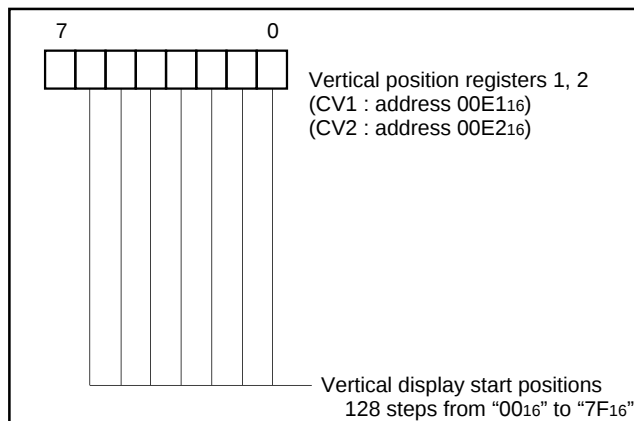
Fig. 36. Structure of vertical position register
