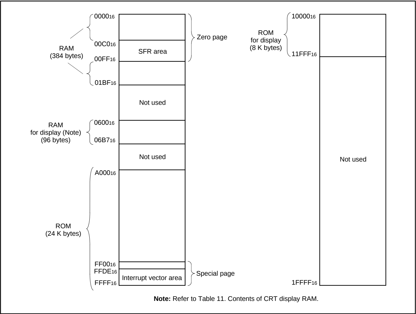
Fig. 2. Memory map
