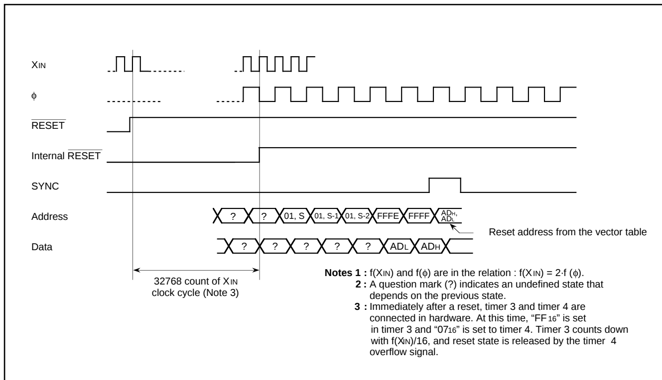
Fig. 49. Reset sequence
