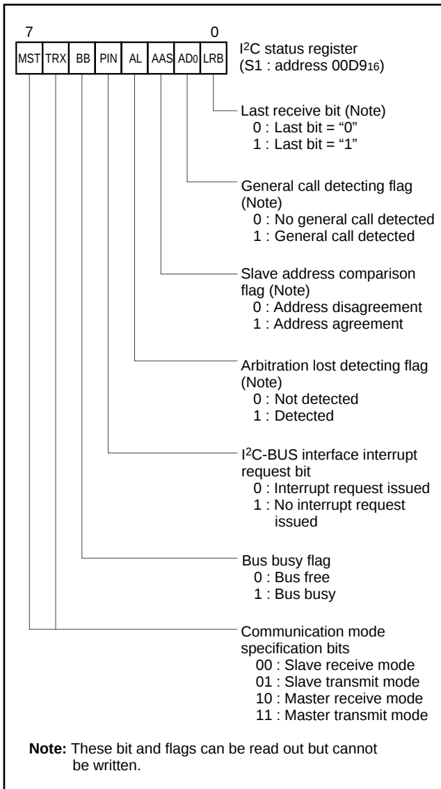
Fig. 17. Structure of I²C status register
