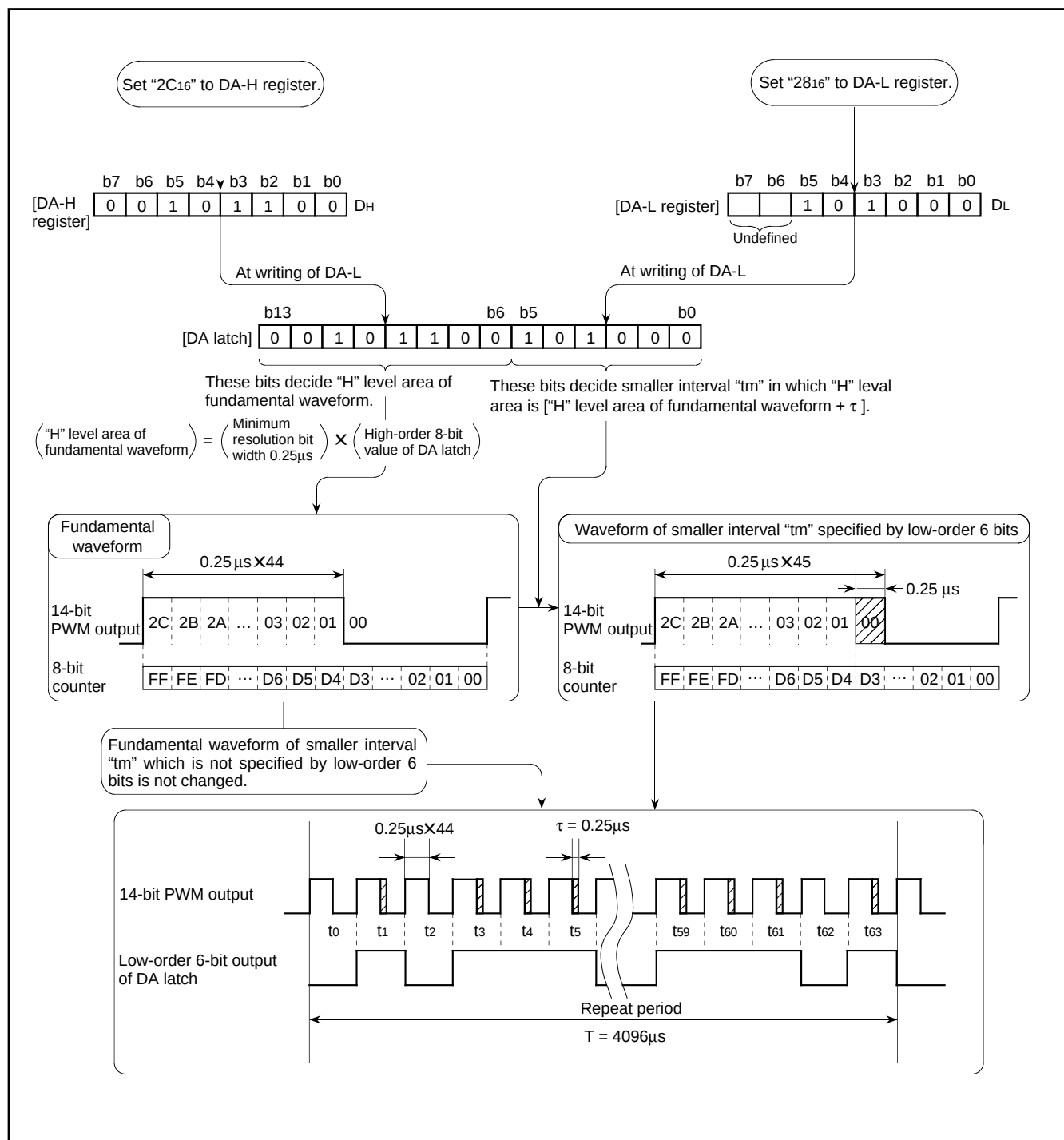
Fig. 25. 14-bit PWM output example ( f(X_{IN}) = 8\text{ MHz} )
