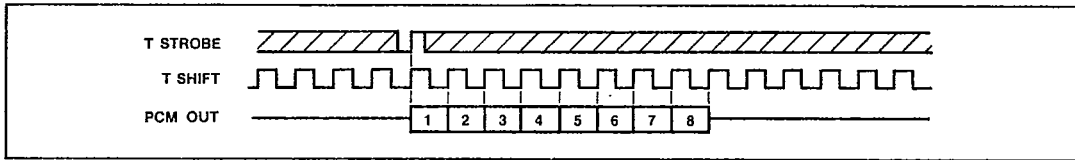
Fig.4 Transmit alignment
