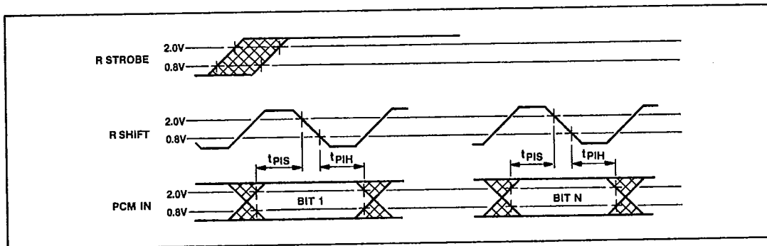
Fig.10 Timing - receive data
