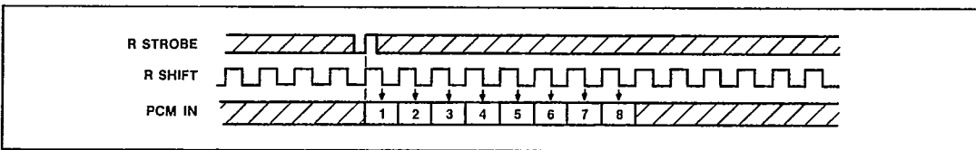
Fig.6 Receive alignment
