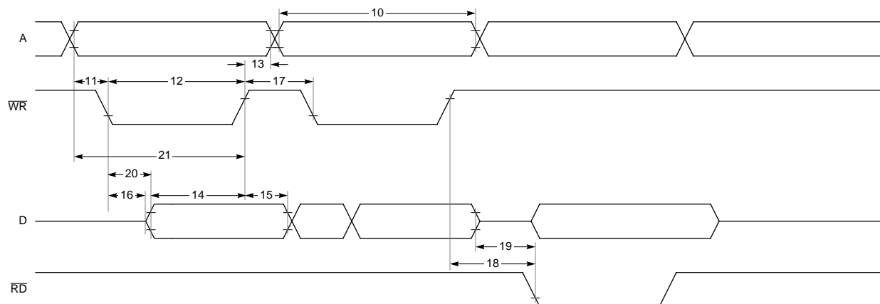
Figure 24. Memory Write
