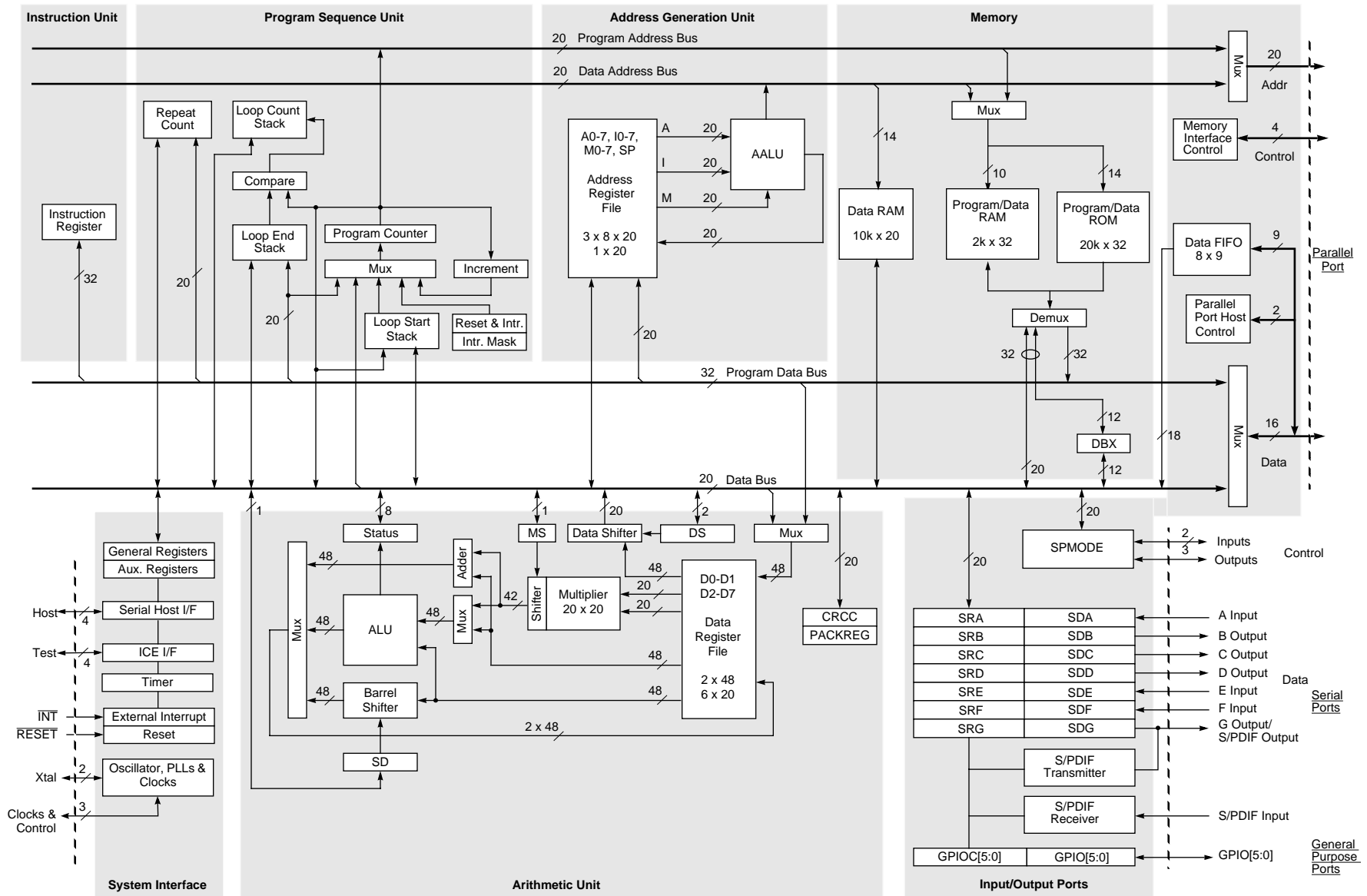
Figure 12. ZR38601 Detailed Block Diagram
