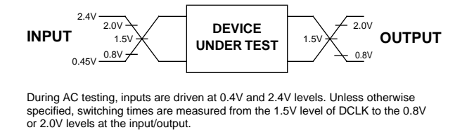
Figure 21. AC Testing Input, Output
