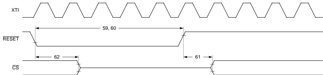
Figure 34. Warm/Cold Reset
