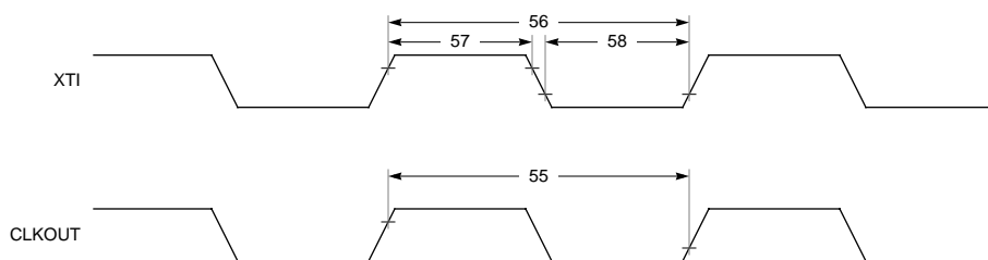
Figure 32. External Clocks
