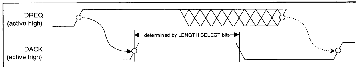
Figure 3-6. Demand Mode Handshaking
