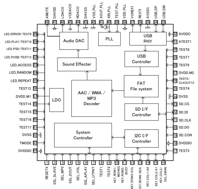
Figure 2. Block diagram
