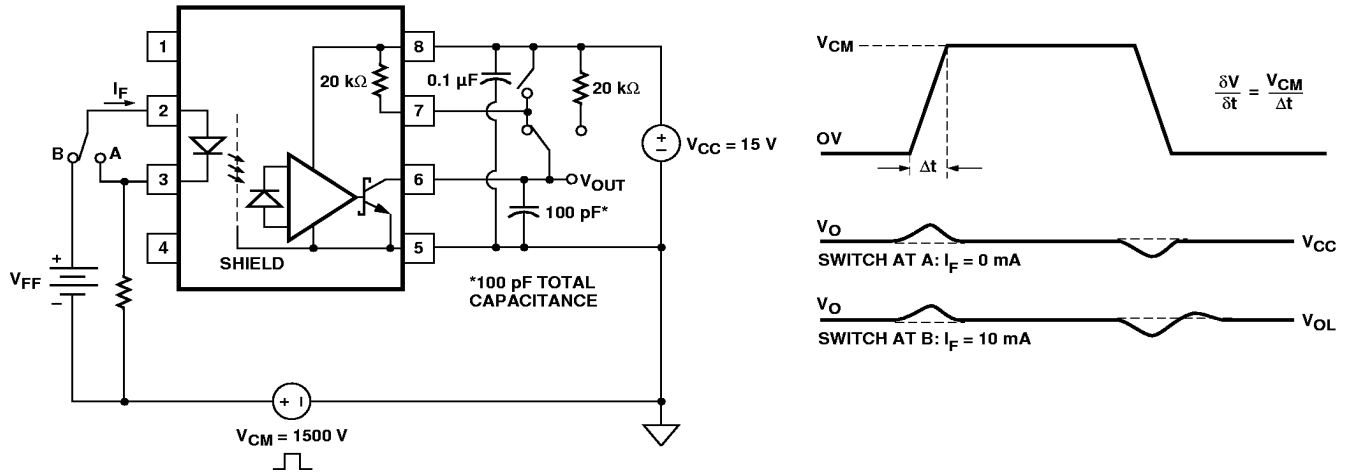
Figure 7. CMR Test Circuit. Typical CMR Waveform.
