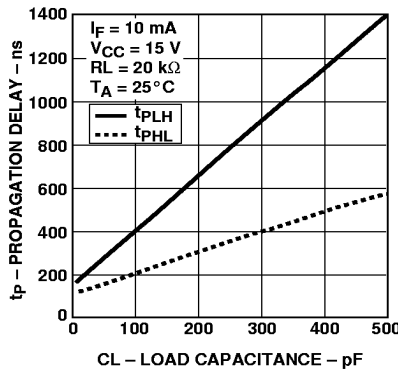
Figure 11. Propagation Delay vs. Load Capacitance.
