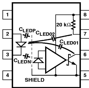
Figure 17. Optocoupler Input to Output Capacitance Model for Shielded Optocouplers.
