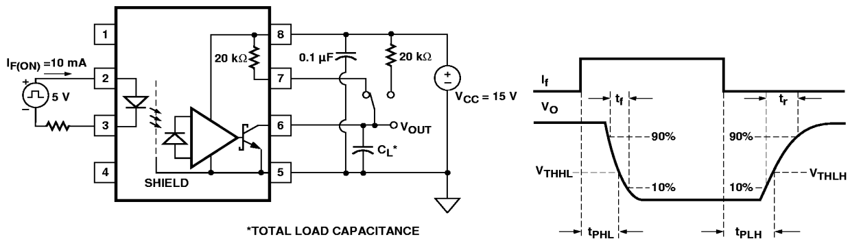
Figure 6. Propagation Delay Test Circuit.
