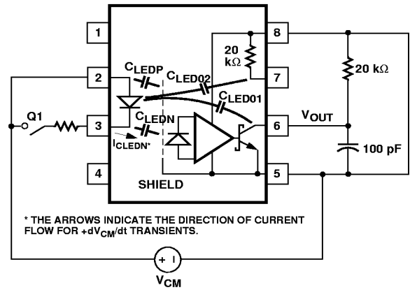
Figure 22. AC Equivalent Circuit for Figure 21 During Common Mode Transients.
