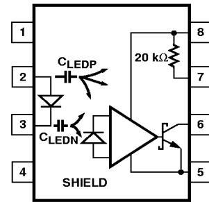
Figure 16. Optocoupler Input to Output Capacitance Model for Unshielded Optocouplers.
