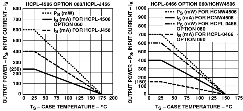
Figure 14. Thermal Derating Curve, Dependence of Safety Limiting Value with Case Temperature per VDE 0884.
