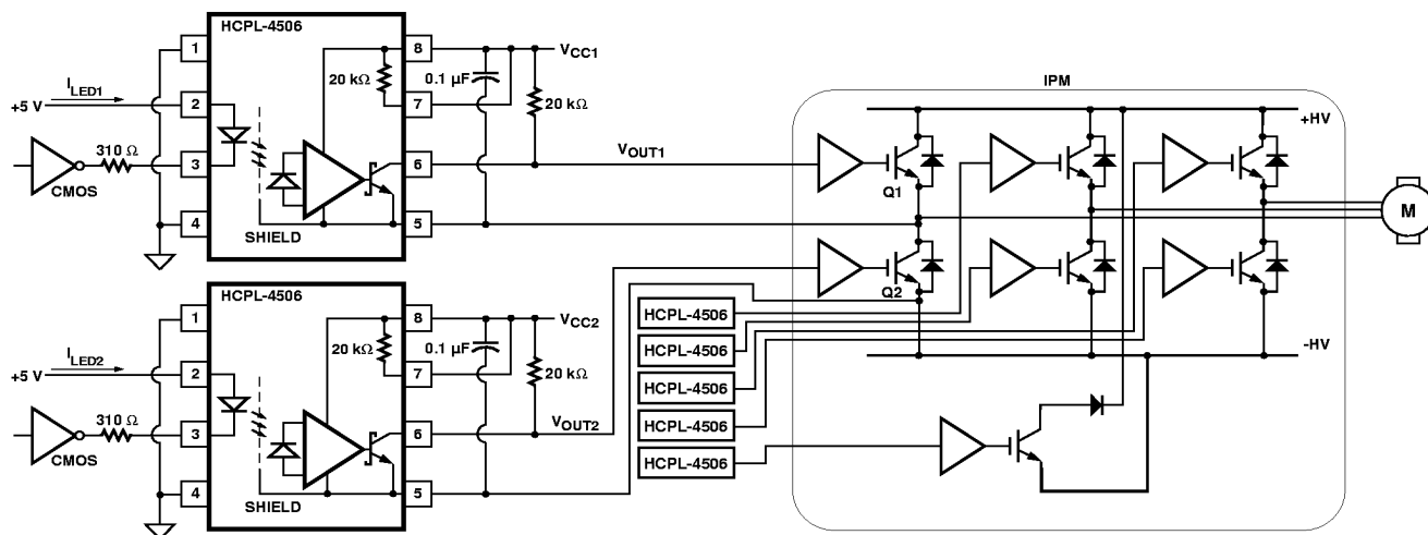
Figure 24. Typical Application Circuit.
