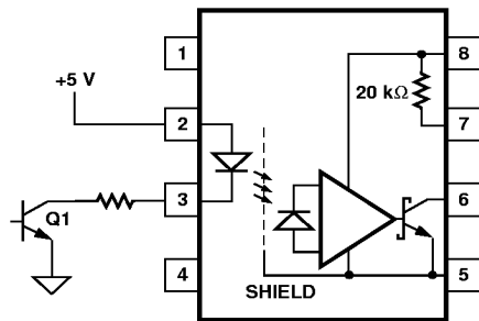
Figure 21. Not Recommended Open Collector LED Drive Circuit.
