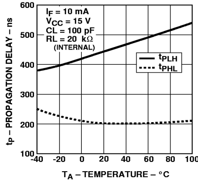
Figure 9. Propagation Delay with Internal 20 kΩ RL vs. Temperature.
