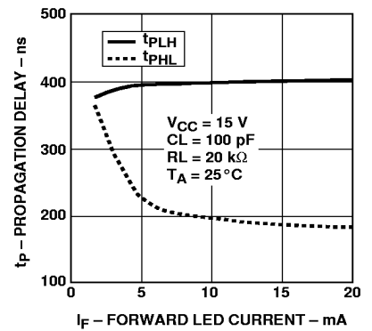
Figure 13. Propagation Delay vs. Input Current.
