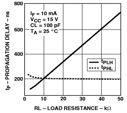
Figure 10. Propagation Delay vs. Load Resistance.
