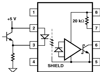
Figure 23. Recommended LED Drive Circuit for Ultra High CMR.
