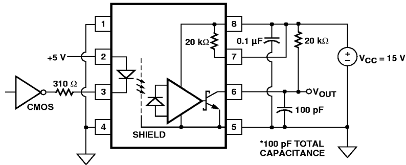
Figure 15. Recommended LED Drive Circuit.
