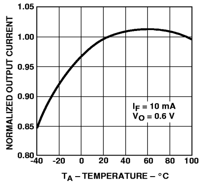
Figure 2. Normalized Output Current vs. Temperature.
