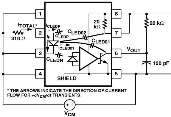
Figure 19. AC Equivalent Circuit for Figure 18 During Common Mode Transients.
