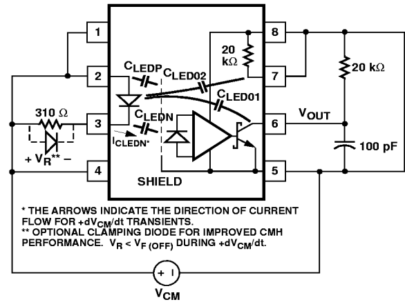
Figure 20. AC Equivalent Circuit for Figure 15 During Common Mode Transients.
