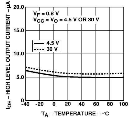
Figure 3. High Level Output Current vs. Temperature.
