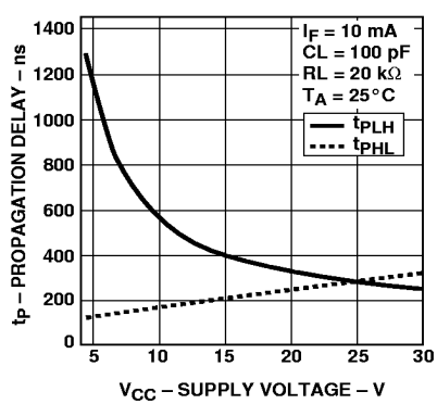
Figure 12. Propagation Delay vs. Supply Voltage.
