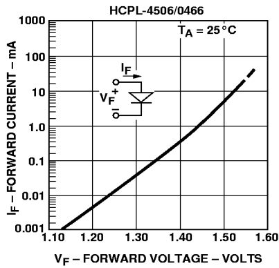
Figure 4. HCPL-4506 and HCPL-0466 Input Current vs. Forward Voltage.
