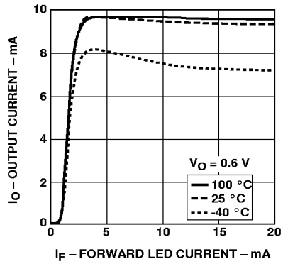
Figure 1. Typical Transfer Characteristics.
