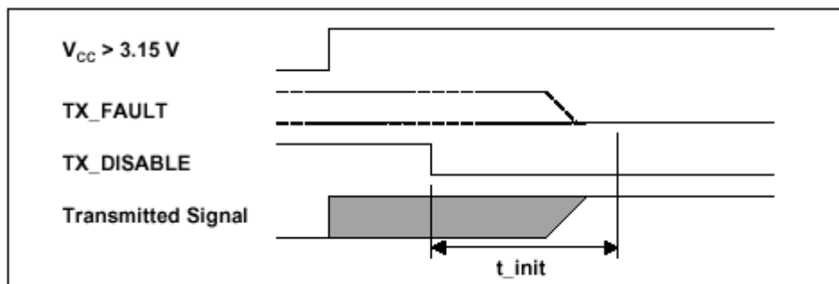
Figure 4. Power on initialization of SFP, Tx Disable asserted
