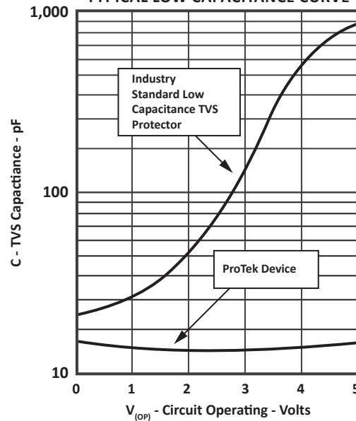
FIGURE 4 TYPICAL LOW CAPACITANCE CURVE
