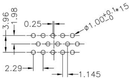
15 Pin Female Connector PCB Pin Layout Scale 2:1
