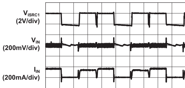
Input vs. Output Transient ( V_{IN} = 2.7V ; Data 1)
