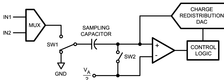
FIGURE 2. ADC122S051 in Hold Mode
