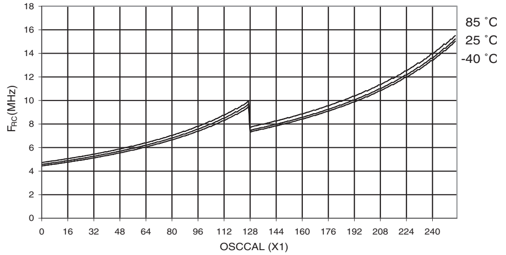
Figure 24-37. Calibrated 1.6 MHz RC Oscillator Frequency vs. V CC
