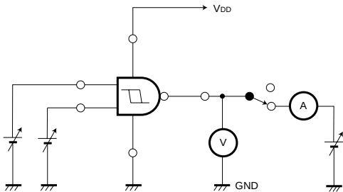
Fig. 1 DC characteristics
