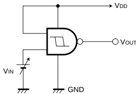
Fig. 3 Hysteresis voltage
