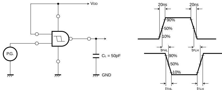
Fig. 2 Switching characteristic
