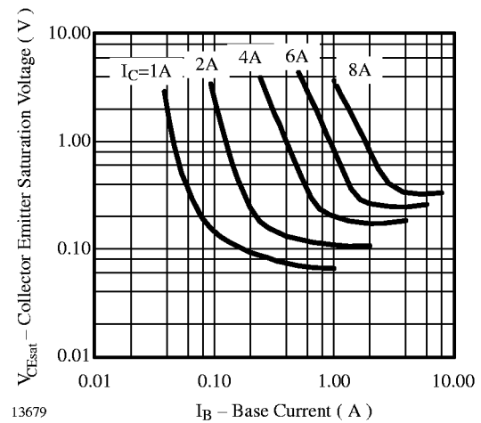
Figure 8. V_{\text{CEsat}} vs. I_B
