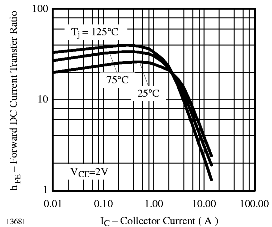
Figure 9. h_{\text{FE}} vs. I_C
